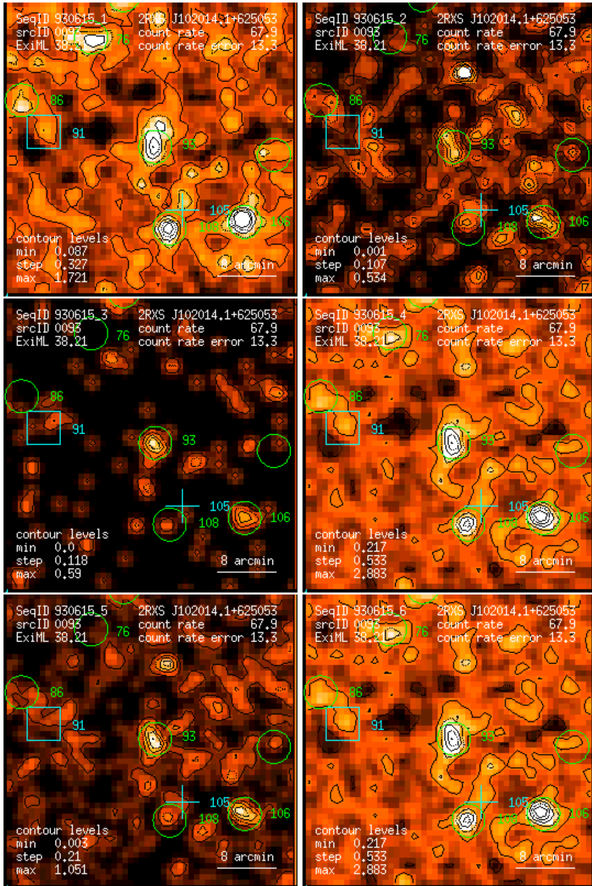
Figure 93: RASS 930615: detection 0093: band rate images, Gaussian filter: (1) PSPC channels 11 – 41, (2) 52 – 90, (3) 91 – 201, (4) 11 – 235, (5) 52 – 201, (6) 11 – 201. Broad band rates in counts/ks. Band rate contour levels in counts/ks/arcmin 2 .
