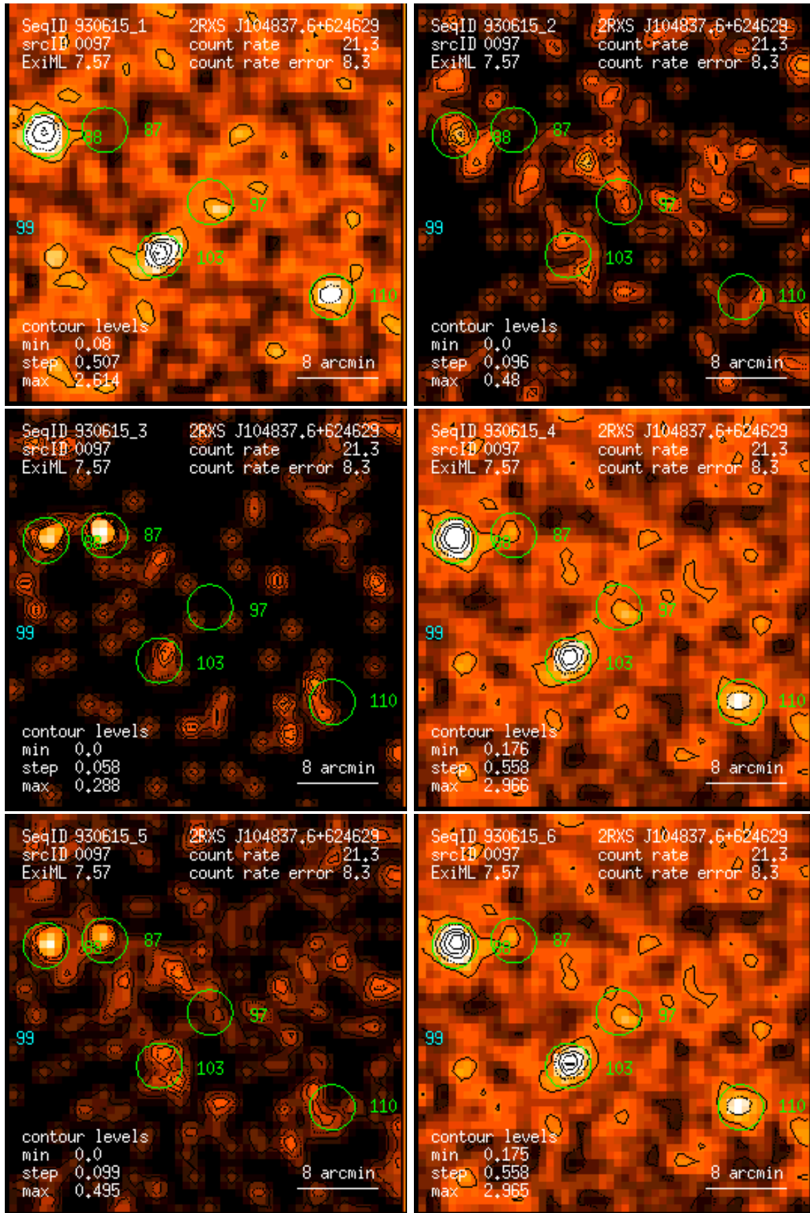
Figure 97: RASS 930615: detection 0097: band rate images, Gaussian filter: (1) PSPC channels 11 – 41, (2) 52 – 90, (3) 91 – 201, (4) 11 – 235, (5) 52 – 201, (6) 11 – 201. Broad band rates in counts/ks. Band rate contour levels in counts/ks/arcmin 2 .
