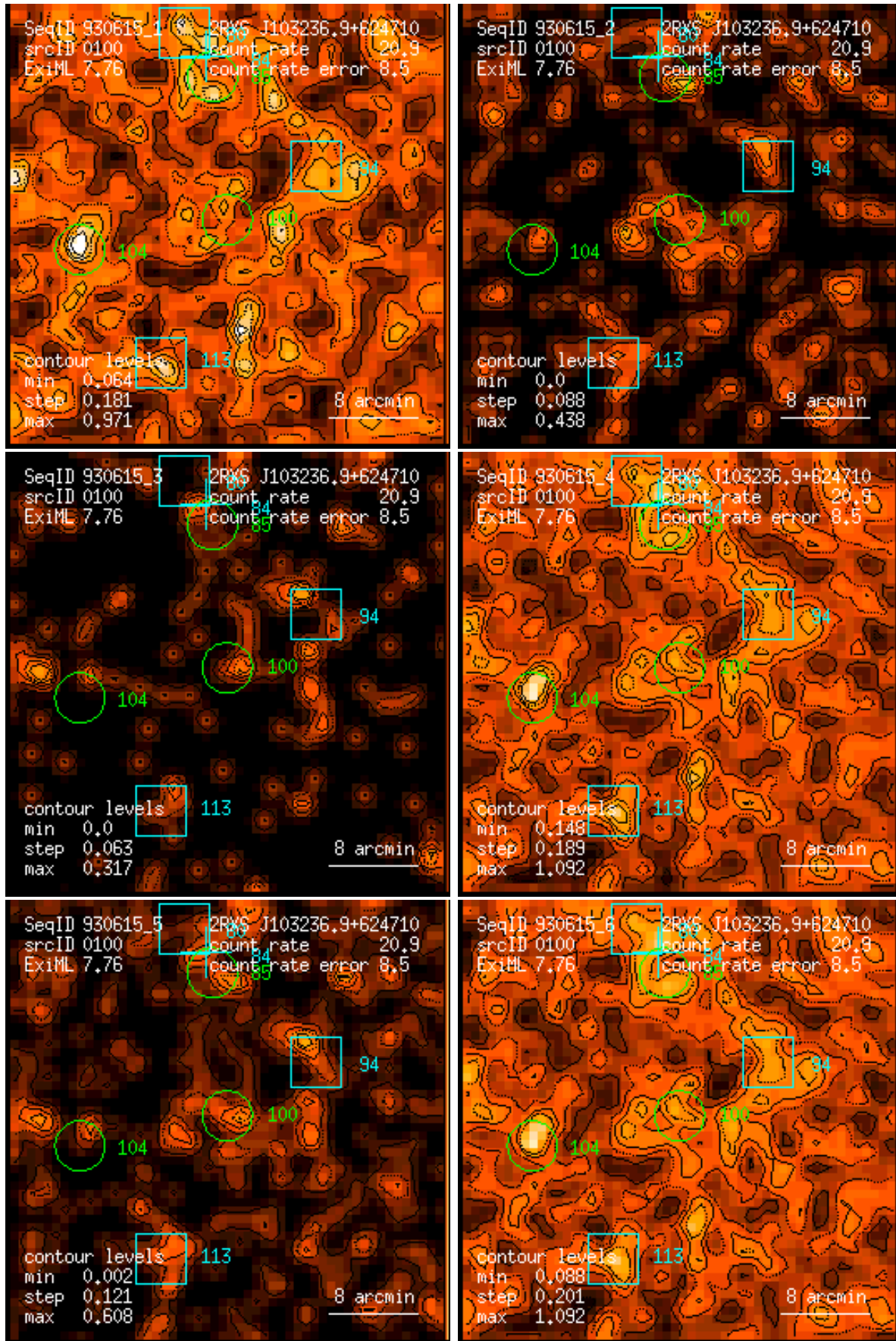
Figure 100: RASS 930615: detection 0100: band rate images, Gaussian filter: (1) PSPC channels 11 – 41, (2) 52 – 90, (3) 91 – 201, (4) 11 – 235, (5) 52 – 201, (6) 11 – 201. Broad band rates in counts/ks. Band rate contour levels in counts/ks/arcmin 2 .
