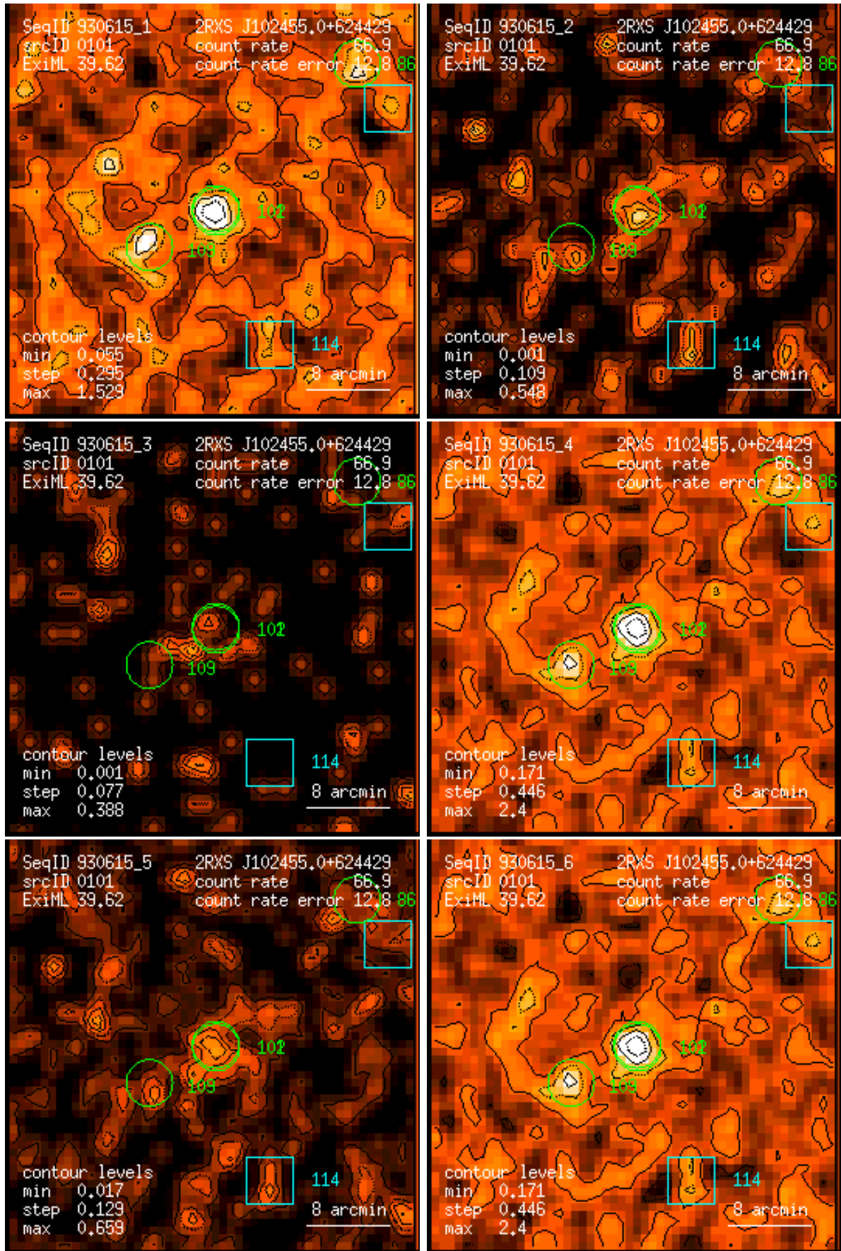
Figure 101: RASS 930615: detection 0101: band rate images, Gaussian filter: (1) PSPC channels 11 – 41, (2) 52 – 90, (3) 91 – 201, (4) 11 – 235, (5) 52 – 201, (6) 11 – 201. Broad band rates in counts/ks. Band rate contour levels in counts/ks/arcmin 2 .
