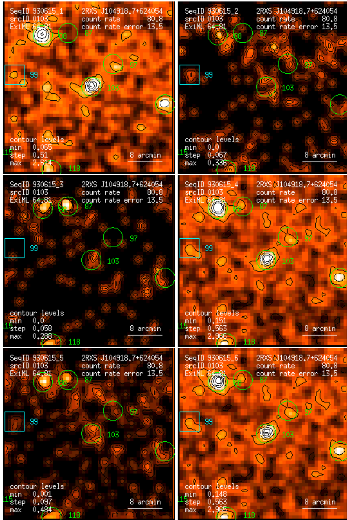
Figure 103: RASS 930615: detection 0103: band rate images, Gaussian filter: (1) PSPC channels 11 – 41, (2) 52 – 90, (3) 91 – 201, (4) 11 – 235, (5) 52 – 201, (6) 11 – 201. Broad band rates in counts/ks. Band rate contour levels in counts/ks/arcmin 2 .
