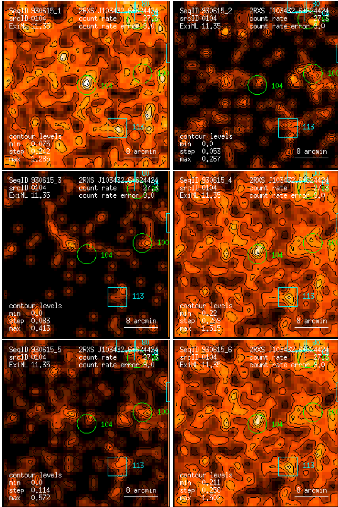
Figure 104: RASS 930615: detection 0104: band rate images, Gaussian filter: (1) PSPC channels 11 – 41, (2) 52 – 90, (3) 91 – 201, (4) 11 – 235, (5) 52 – 201, (6) 11 – 201. Broad band rates in counts/ks. Band rate contour levels in counts/ks/arcmin 2 .
