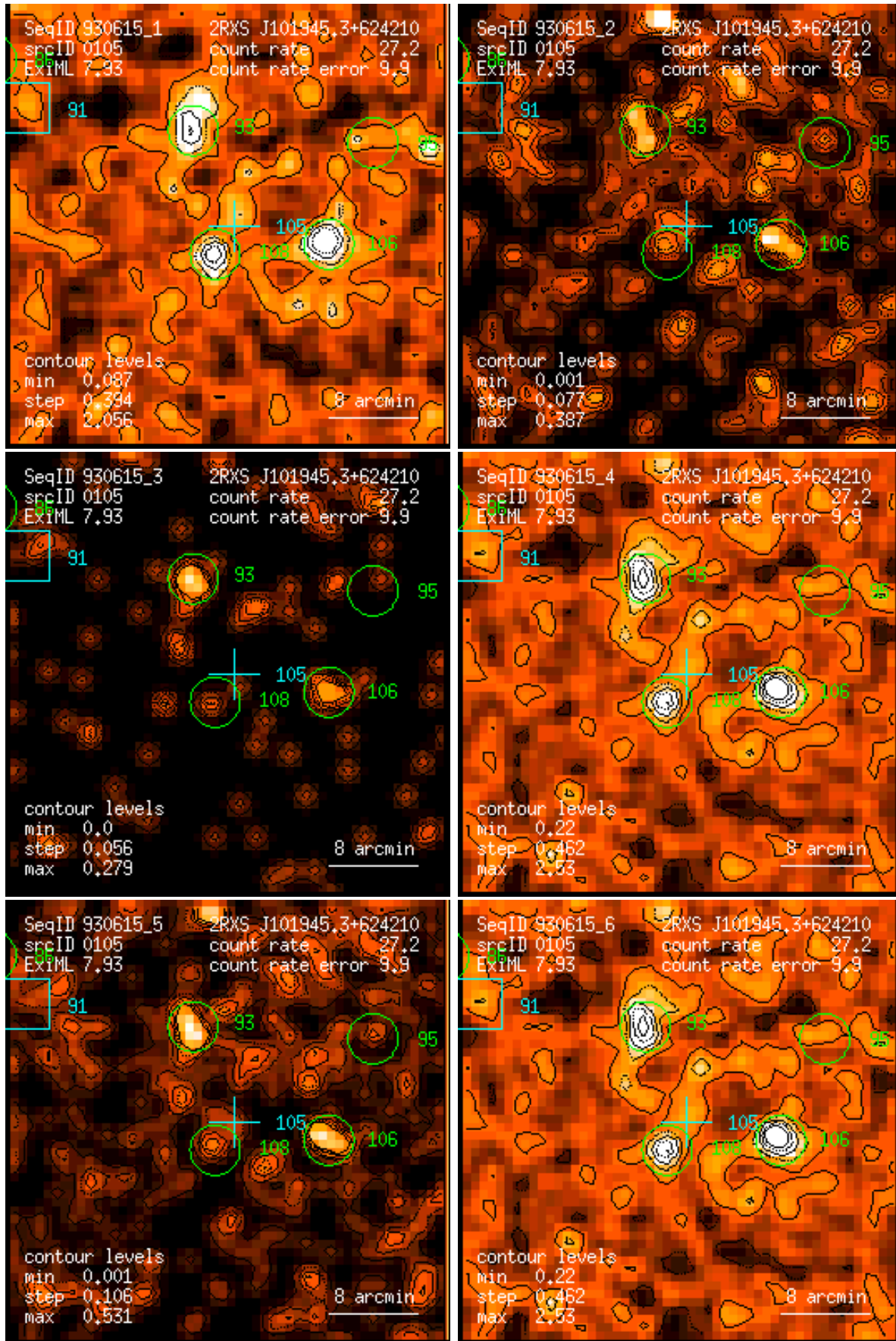
Figure 105: RASS 930615: detection 0105: band rate images, Gaussian filter: (1) PSPC channels 11 – 41, (2) 52 – 90, (3) 91 – 201, (4) 11 – 235, (5) 52 – 201, (6) 11 – 201. Broad band rates in counts/ks. Band rate contour levels in counts/ks/arcmin 2 .
