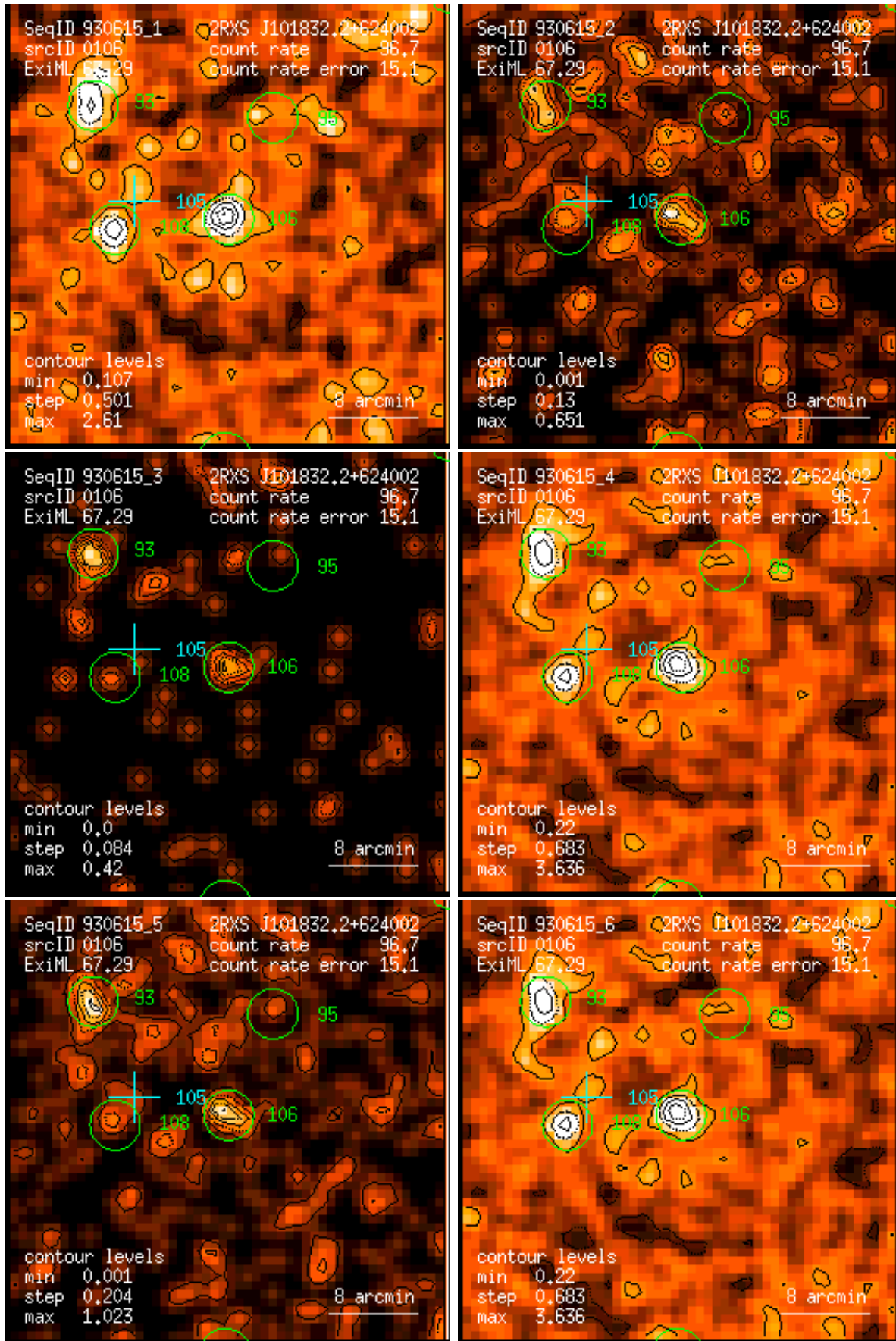
Figure 106: RASS 930615: detection 0106: band rate images, Gaussian filter: (1) PSPC channels 11 – 41, (2) 52 – 90, (3) 91 – 201, (4) 11 – 235, (5) 52 – 201, (6) 11 – 201. Broad band rates in counts/ks. Band rate contour levels in counts/ks/arcmin 2 .
