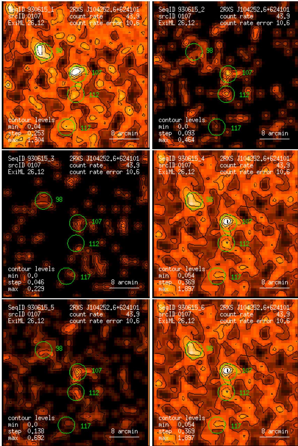
Figure 107: RASS 930615: detection 0107: band rate images, Gaussian filter: (1) PSPC channels 11 – 41, (2) 52 – 90, (3) 91 – 201, (4) 11 – 235, (5) 52 – 201, (6) 11 – 201. Broad band rates in counts/ks. Band rate contour levels in counts/ks/arcmin 2 .
