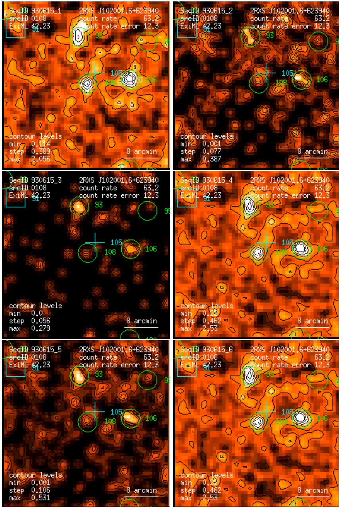
Figure 108: RASS 930615: detection 0108: band rate images, Gaussian filter: (1) PSPC channels 11 – 41, (2) 52 – 90, (3) 91 – 201, (4) 11 – 235, (5) 52 – 201, (6) 11 – 201. Broad band rates in counts/ks. Band rate contour levels in counts/ks/arcmin 2 .
