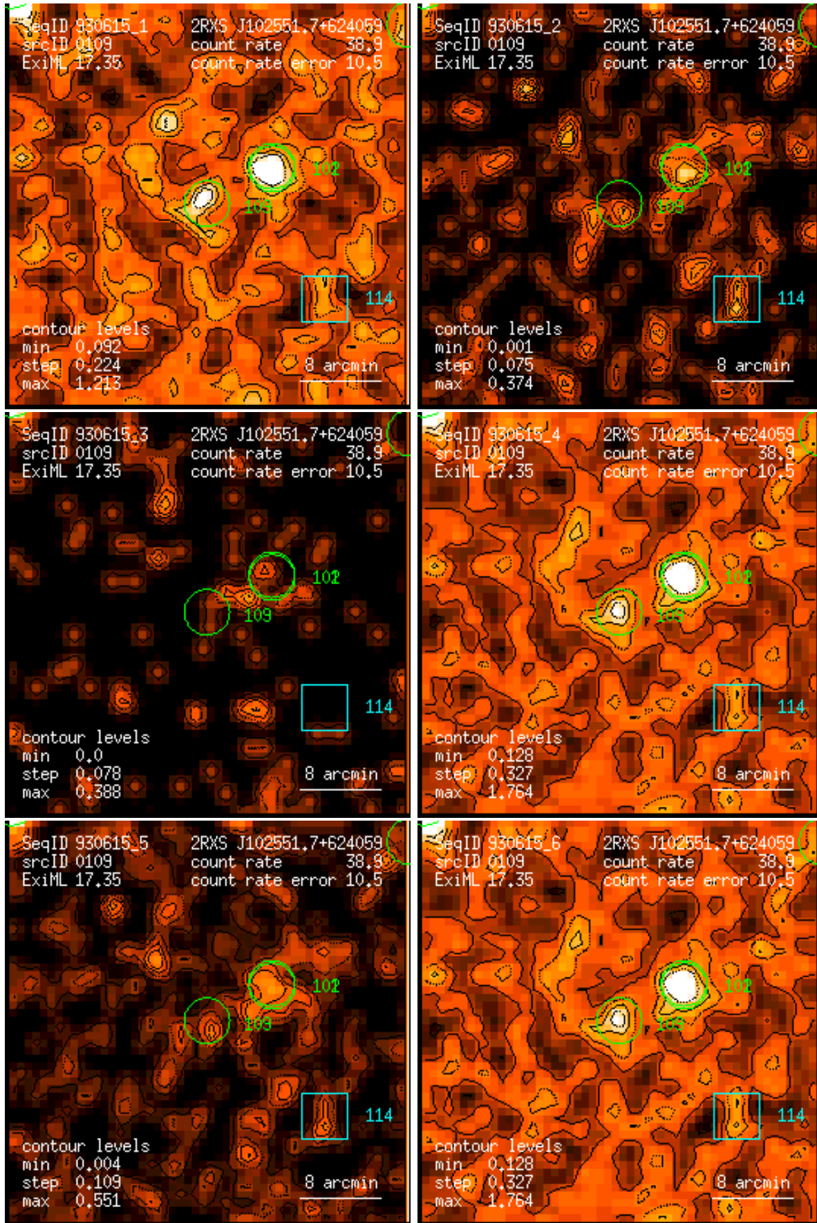
Figure 109: RASS 930615: detection 0109: band rate images, Gaussian filter: (1) PSPC channels 11 – 41, (2) 52 – 90, (3) 91 – 201, (4) 11 – 235, (5) 52 – 201, (6) 11 – 201. Broad band rates in counts/ks. Band rate contour levels in counts/ks/arcmin 2 .
