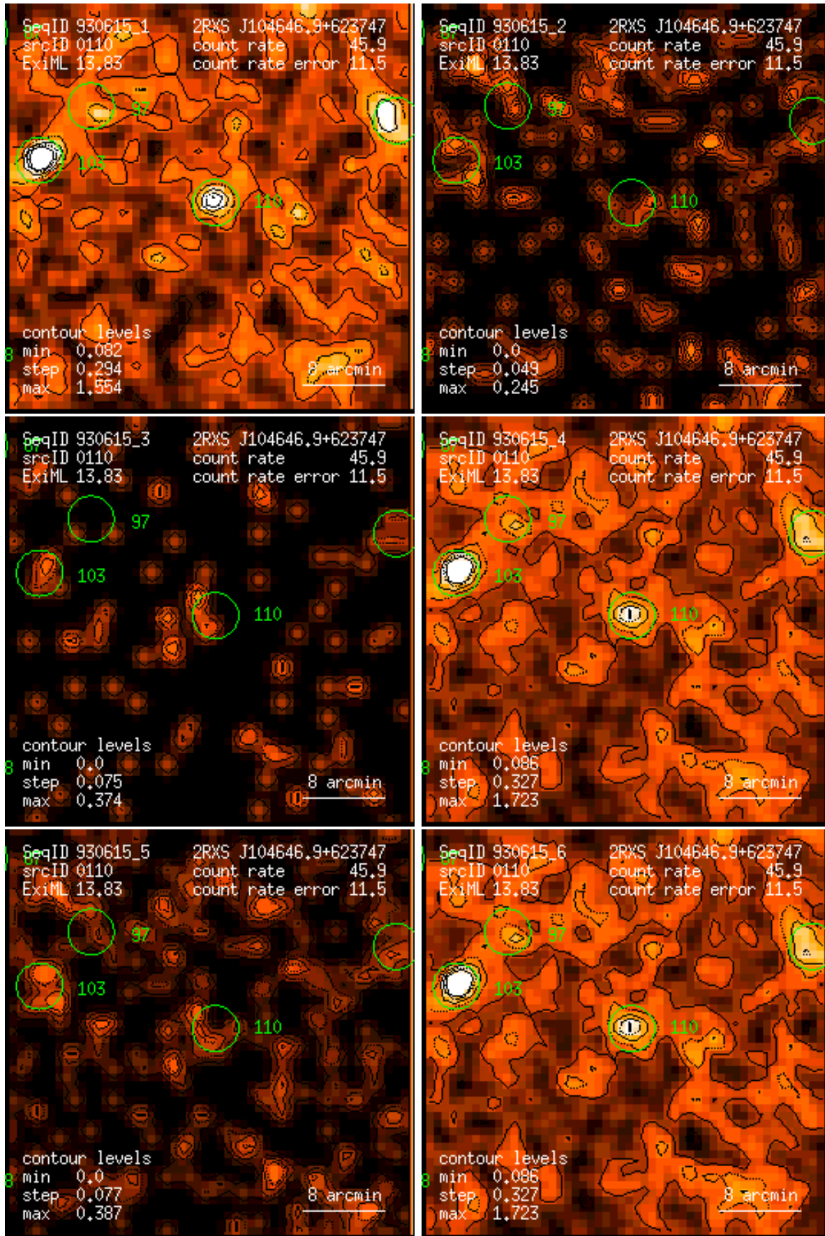
Figure 110: RASS 930615: detection 0110: band rate images, Gaussian filter: (1) PSPC channels 11 – 41, (2) 52 – 90, (3) 91 – 201, (4) 11 – 235, (5) 52 – 201, (6) 11 – 201. Broad band rates in counts/ks. Band rate contour levels in counts/ks/arcmin 2 .
