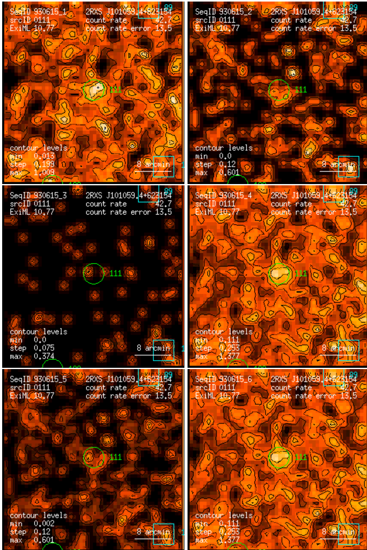
Figure 111: RASS 930615: detection 0111: band rate images, Gaussian filter: (1) PSPC channels 11 – 41, (2) 52 – 90, (3) 91 – 201, (4) 11 – 235, (5) 52 – 201, (6) 11 – 201. Broad band rates in counts/ks. Band rate contour levels in counts/ks/arcmin 2 .
