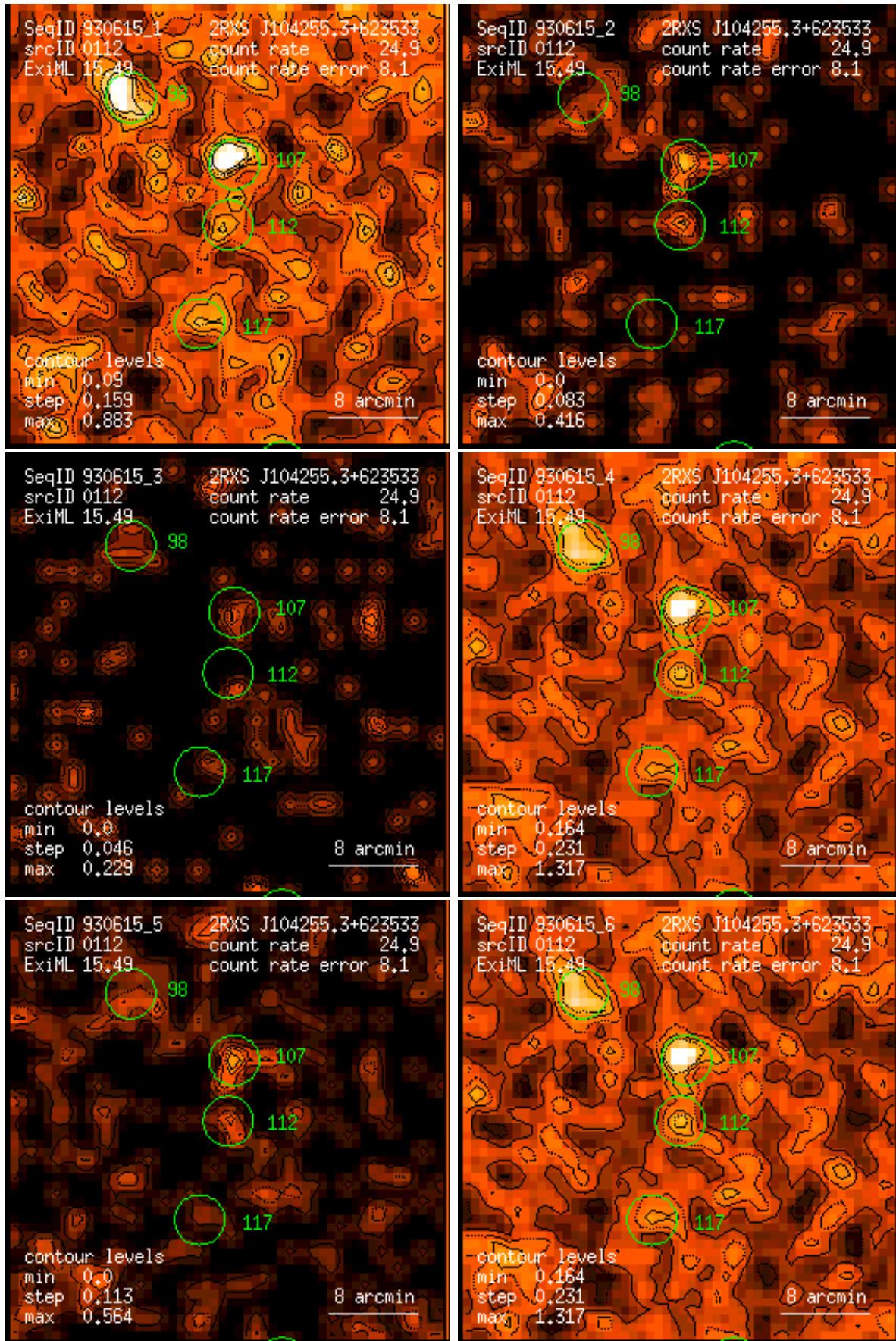
Figure 112: RASS 930615: detection 0112: band rate images, Gaussian filter: (1) PSPC channels 11 – 41, (2) 52 – 90, (3) 91 – 201, (4) 11 – 235, (5) 52 – 201, (6) 11 – 201. Broad band rates in counts/ks. Band rate contour levels in counts/ks/arcmin 2 .
