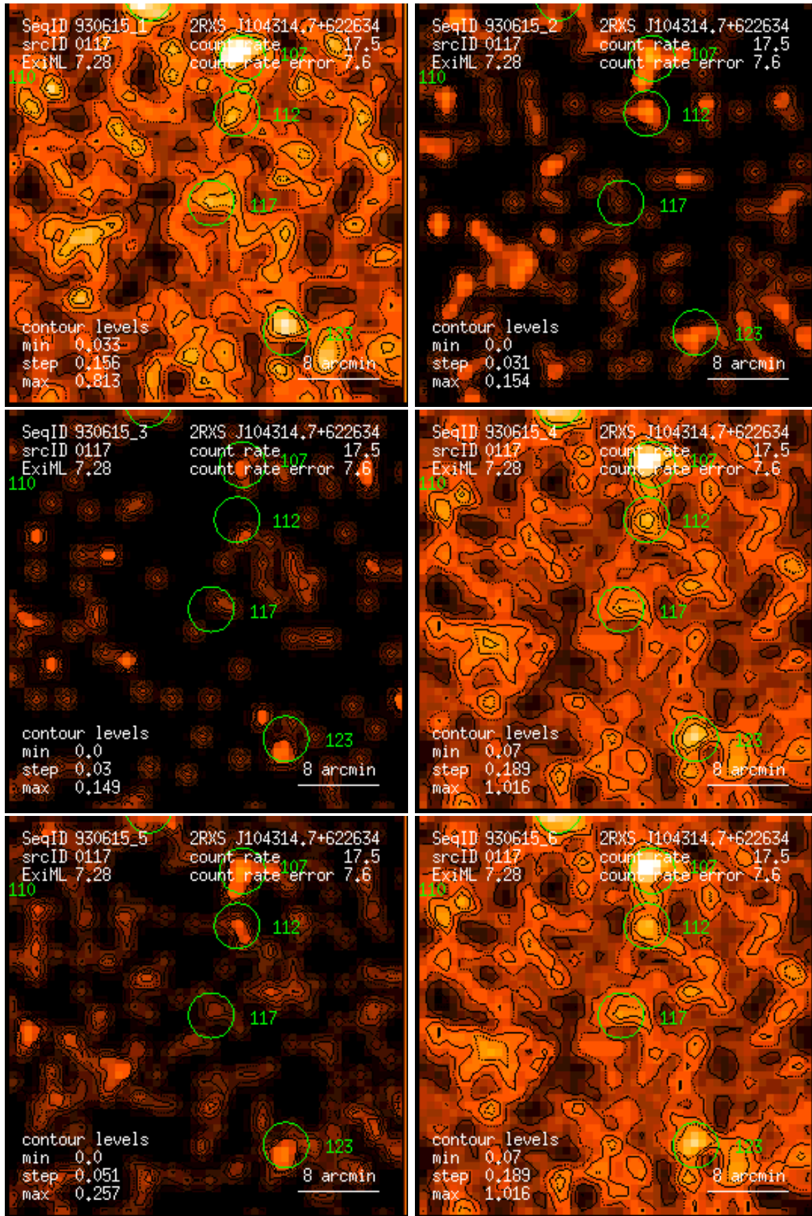
Figure 117: RASS 930615: detection 0117: band rate images, Gaussian filter: (1) PSPC channels 11 – 41, (2) 52 – 90, (3) 91 – 201, (4) 11 – 235, (5) 52 – 201, (6) 11 – 201. Broad band rates in counts/ks. Band rate contour levels in counts/ks/arcmin 2 .
