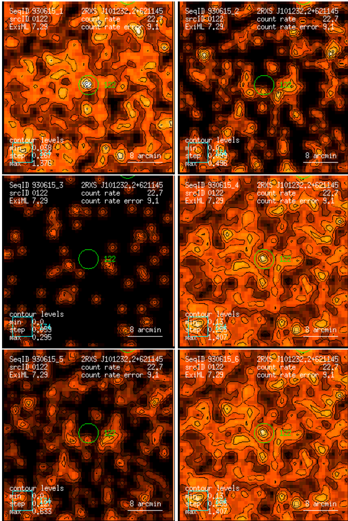
Figure 122: RASS 930615: detection 0122: band rate images, Gaussian filter: (1) PSPC channels 11 – 41, (2) 52 – 90, (3) 91 – 201, (4) 11 – 235, (5) 52 – 201, (6) 11 – 201. Broad band rates in counts/ks. Band rate contour levels in counts/ks/arcmin 2 .
