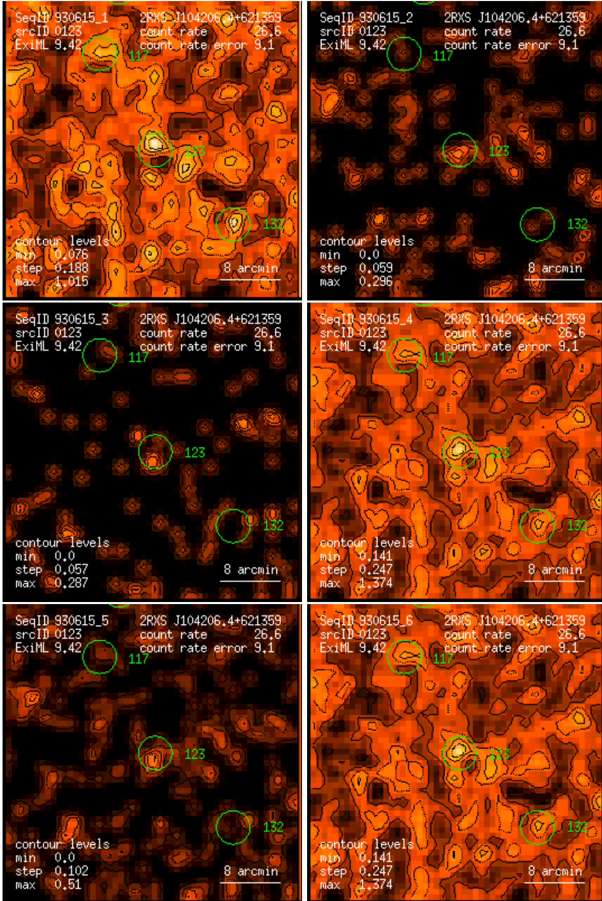
Figure 123: RASS 930615: detection 0123: band rate images, Gaussian filter: (1) PSPC channels 11 – 41, (2) 52 – 90, (3) 91 – 201, (4) 11 – 235, (5) 52 – 201, (6) 11 – 201. Broad band rates in counts/ks. Band rate contour levels in counts/ks/arcmin 2 .
