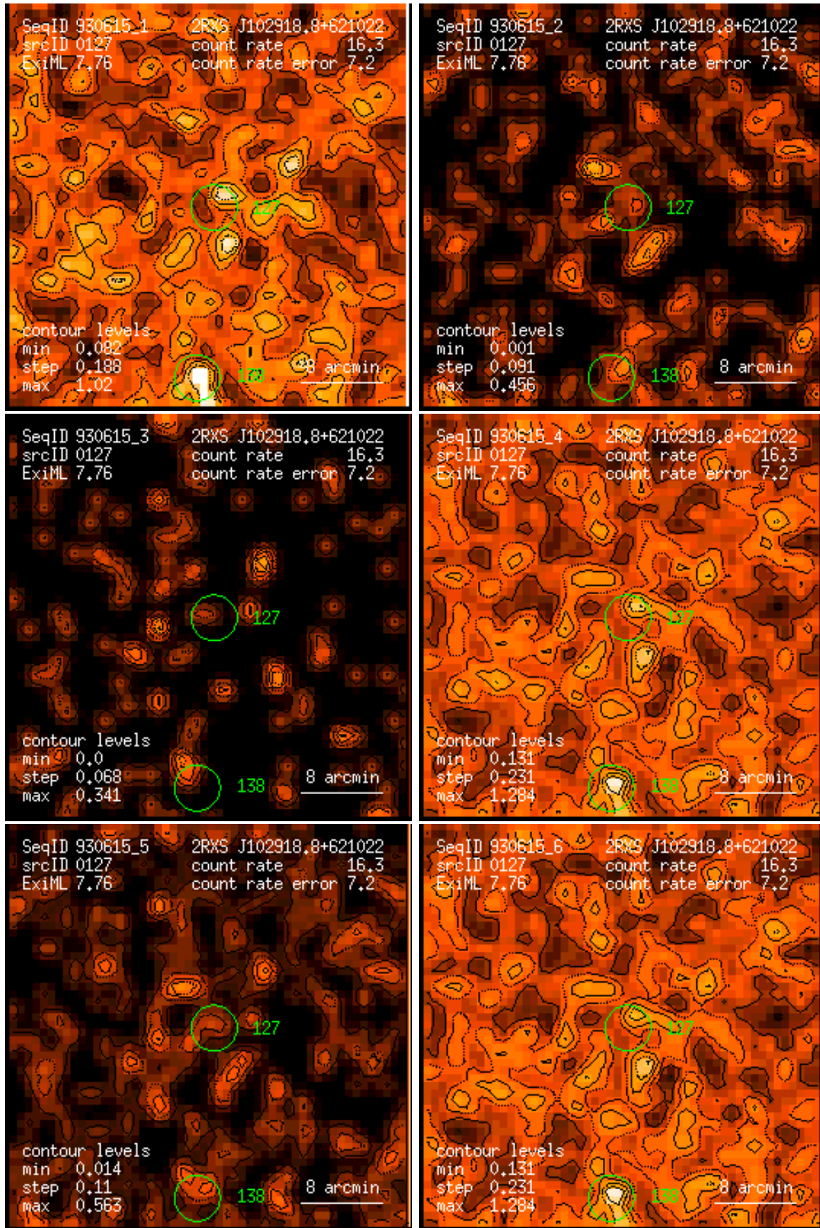
Figure 127: RASS 930615: detection 0127: band rate images, Gaussian filter: (1) PSPC channels 11 – 41, (2) 52 – 90, (3) 91 – 201, (4) 11 – 235, (5) 52 – 201, (6) 11 – 201. Broad band rates in counts/ks. Band rate contour levels in counts/ks/arcmin 2 .
