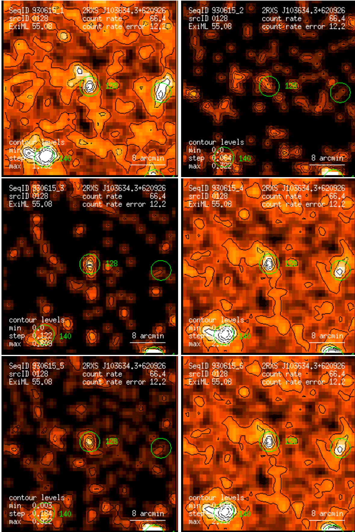
Figure 128: RASS 930615: detection 0128: band rate images, Gaussian filter: (1) PSPC channels 11 – 41, (2) 52 – 90, (3) 91 – 201, (4) 11 – 235, (5) 52 – 201, (6) 11 – 201. Broad band rates in counts/ks. Band rate contour levels in counts/ks/arcmin 2 .
