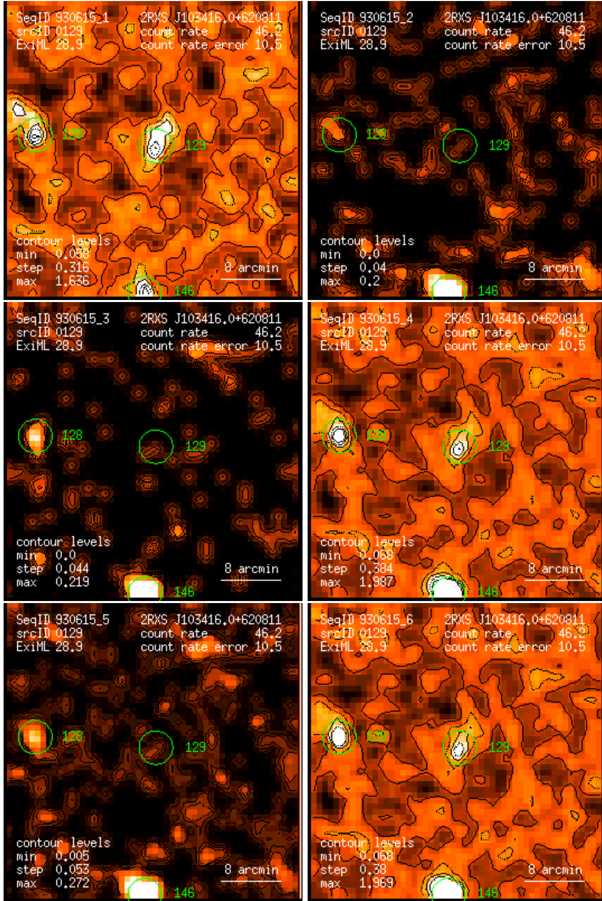
Figure 129: RASS 930615: detection 0129: band rate images, Gaussian filter: (1) PSPC channels 11 – 41, (2) 52 – 90, (3) 91 – 201, (4) 11 – 235, (5) 52 – 201, (6) 11 – 201. Broad band rates in counts/ks. Band rate contour levels in counts/ks/arcmin 2 .
