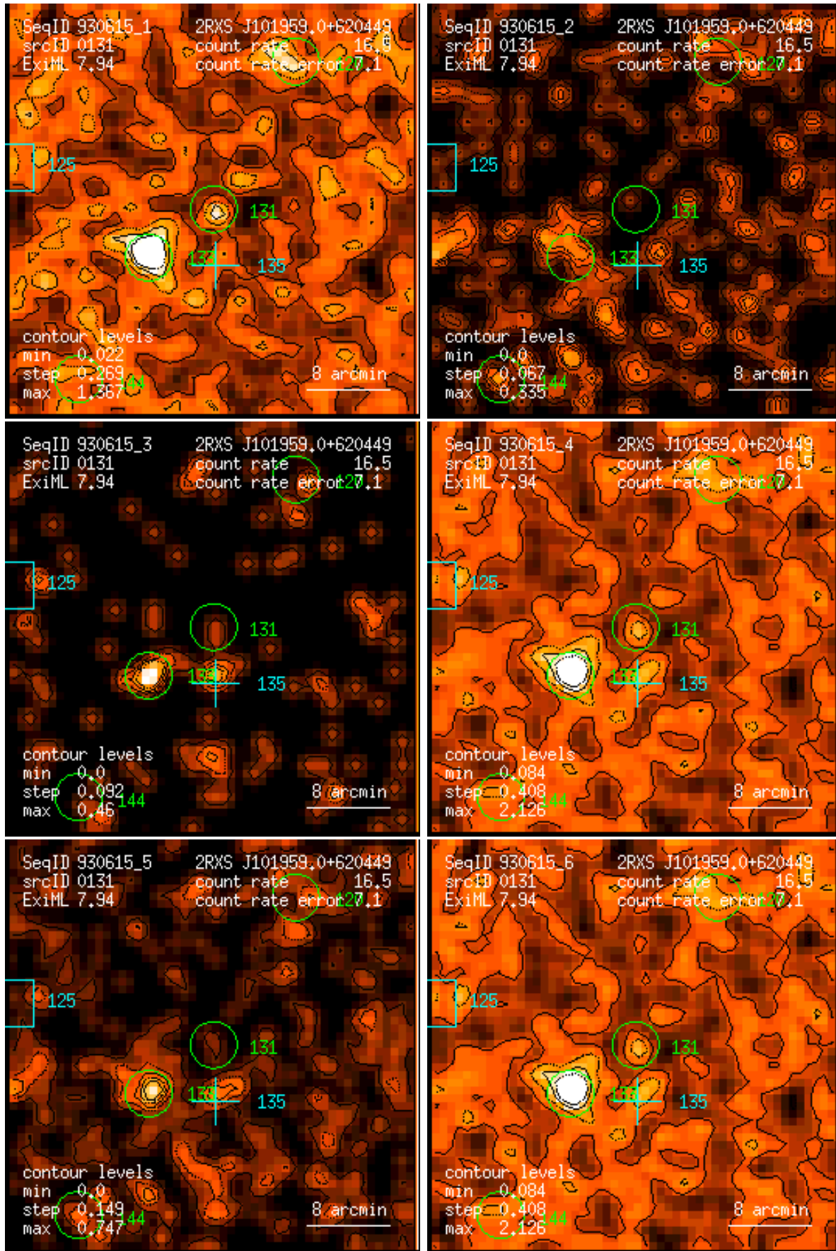
Figure 131: RASS 930615: detection 0131: band rate images, Gaussian filter: (1) PSPC channels 11 – 41, (2) 52 – 90, (3) 91 – 201, (4) 11 – 235, (5) 52 – 201, (6) 11 – 201. Broad band rates in counts/ks. Band rate contour levels in counts/ks/arcmin 2 .
