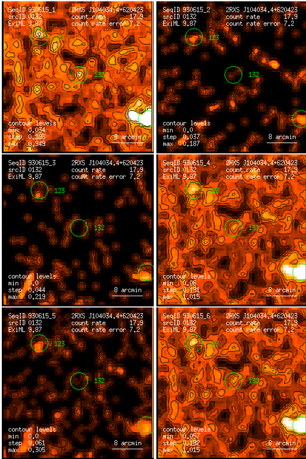
Figure 132: RASS 930615: detection 0132: band rate images, Gaussian filter: (1) PSPC channels 11 – 41, (2) 52 – 90, (3) 91 – 201, (4) 11 – 235, (5) 52 – 201, (6) 11 – 201. Broad band rates in counts/ks. Band rate contour levels in counts/ks/arcmin 2 .
