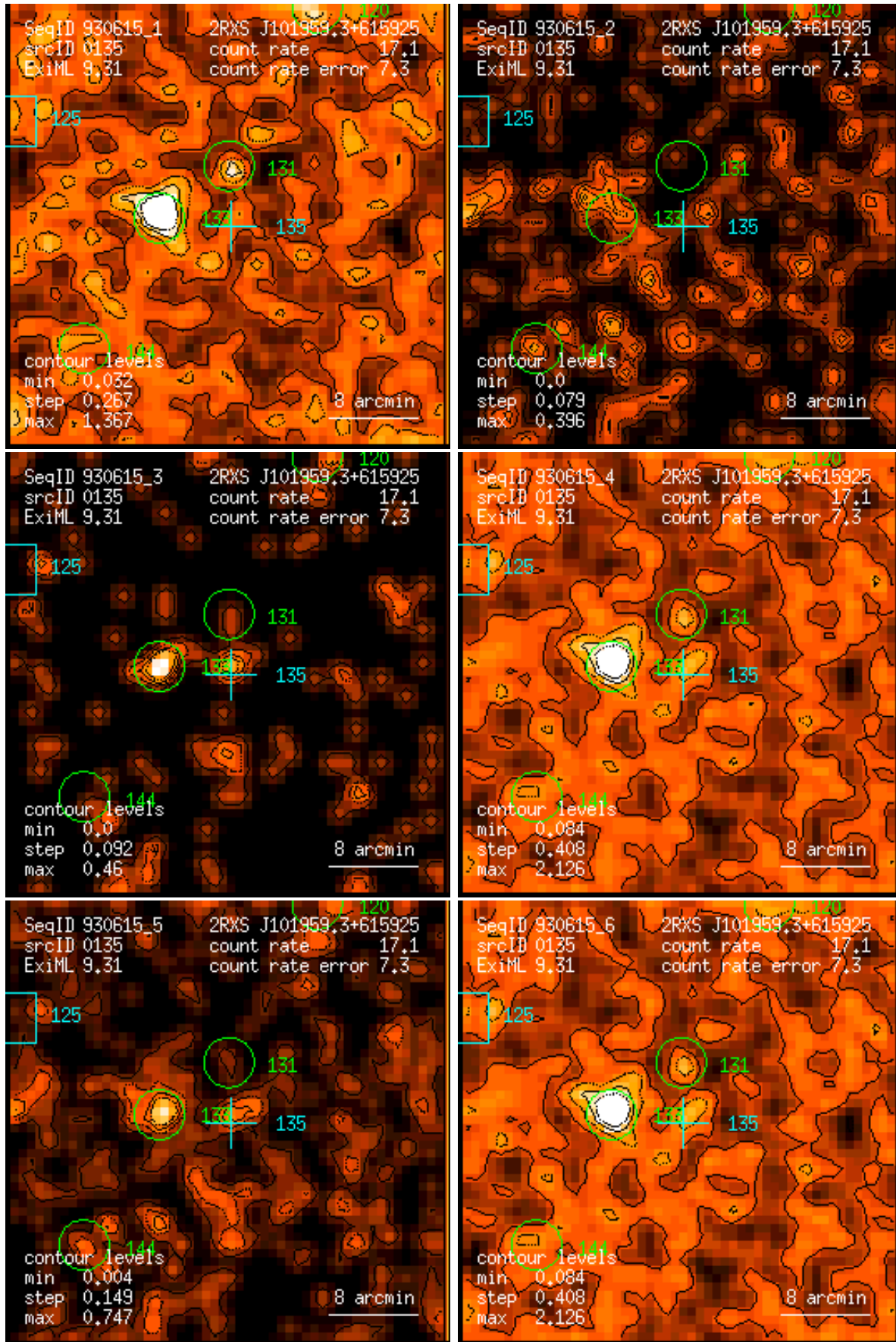
Figure 135: RASS 930615: detection 0135: band rate images, Gaussian filter: (1) PSPC channels 11 – 41, (2) 52 – 90, (3) 91 – 201, (4) 11 – 235, (5) 52 – 201, (6) 11 – 201. Broad band rates in counts/ks. Band rate contour levels in counts/ks/arcmin 2 .
