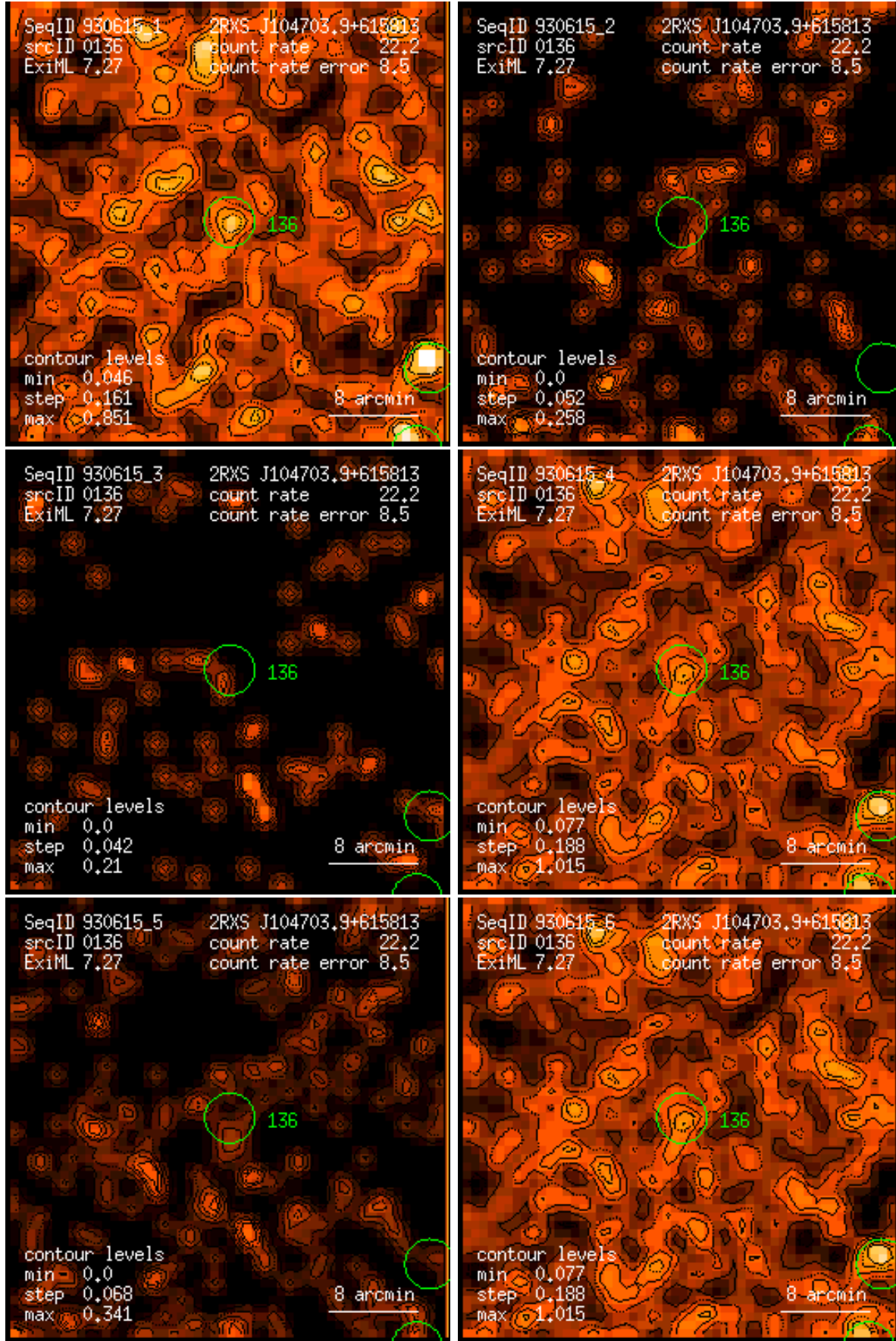
Figure 136: RASS 930615: detection 0136: band rate images, Gaussian filter: (1) PSPC channels 11 – 41, (2) 52 – 90, (3) 91 – 201, (4) 11 – 235, (5) 52 – 201, (6) 11 – 201. Broad band rates in counts/ks. Band rate contour levels in counts/ks/arcmin 2 .
