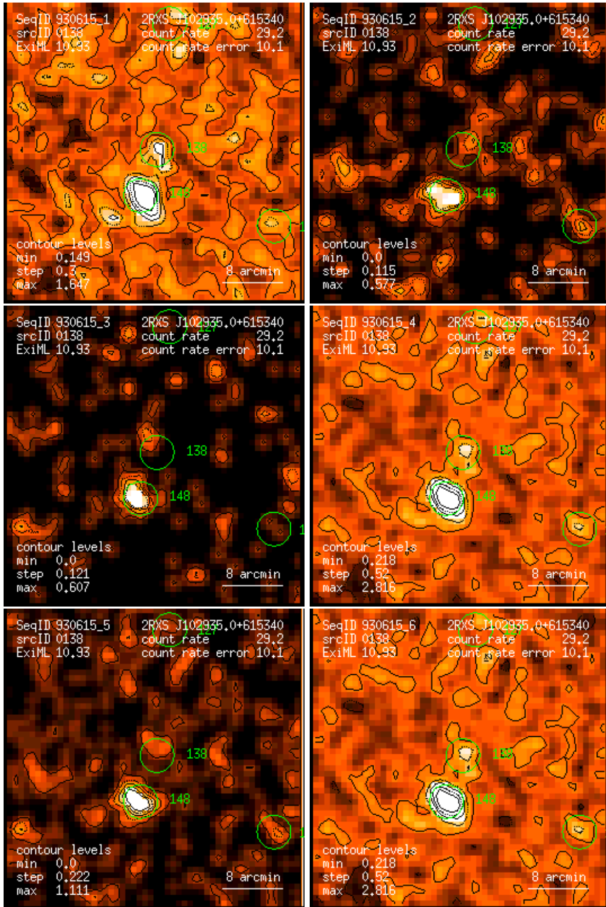
Figure 138: RASS 930615: detection 0138: band rate images, Gaussian filter: (1) PSPC channels 11 – 41, (2) 52 – 90, (3) 91 – 201, (4) 11 – 235, (5) 52 – 201, (6) 11 – 201. Broad band rates in counts/ks. Band rate contour levels in counts/ks/arcmin 2 .
