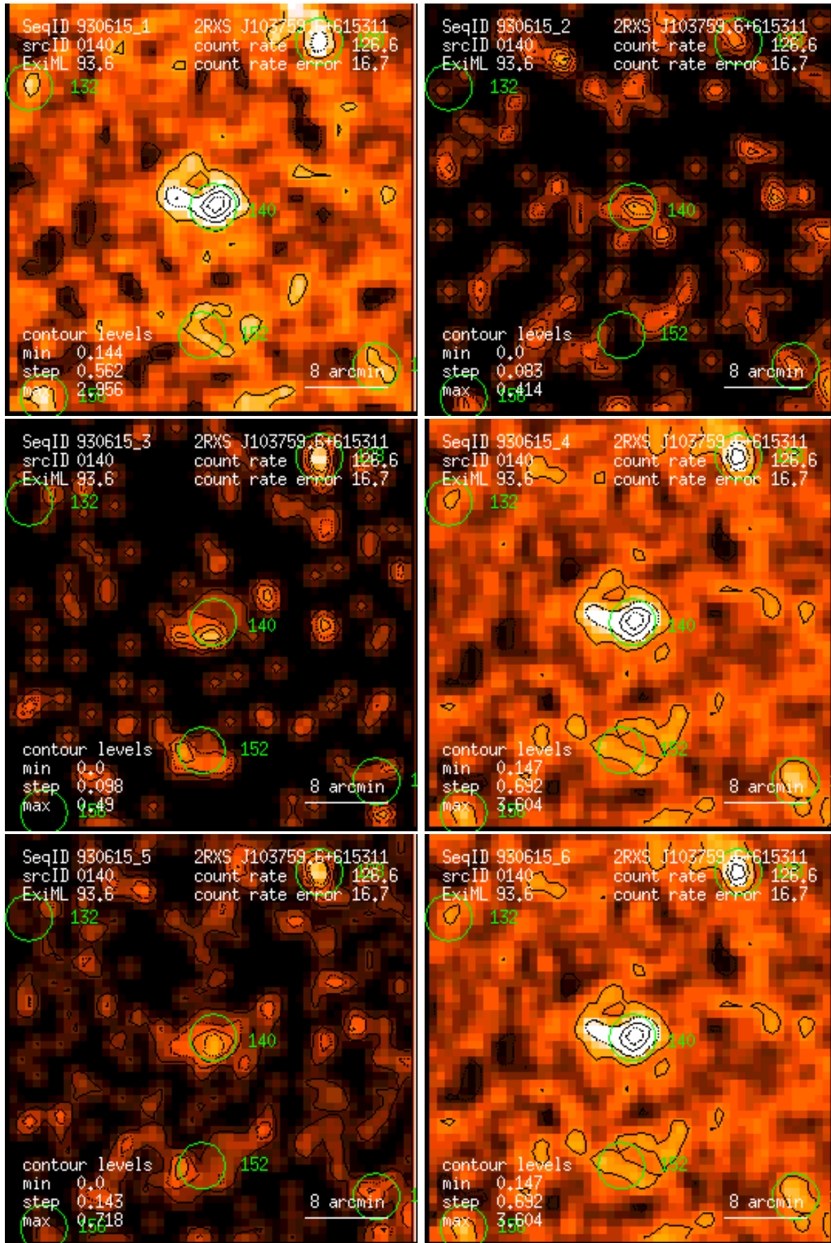
Figure 140: RASS 930615: detection 0140: band rate images, Gaussian filter: (1) PSPC channels 11 – 41, (2) 52 – 90, (3) 91 – 201, (4) 11 – 235, (5) 52 – 201, (6) 11 – 201. Broad band rates in counts/ks. Band rate contour levels in counts/ks/arcmin 2 .
