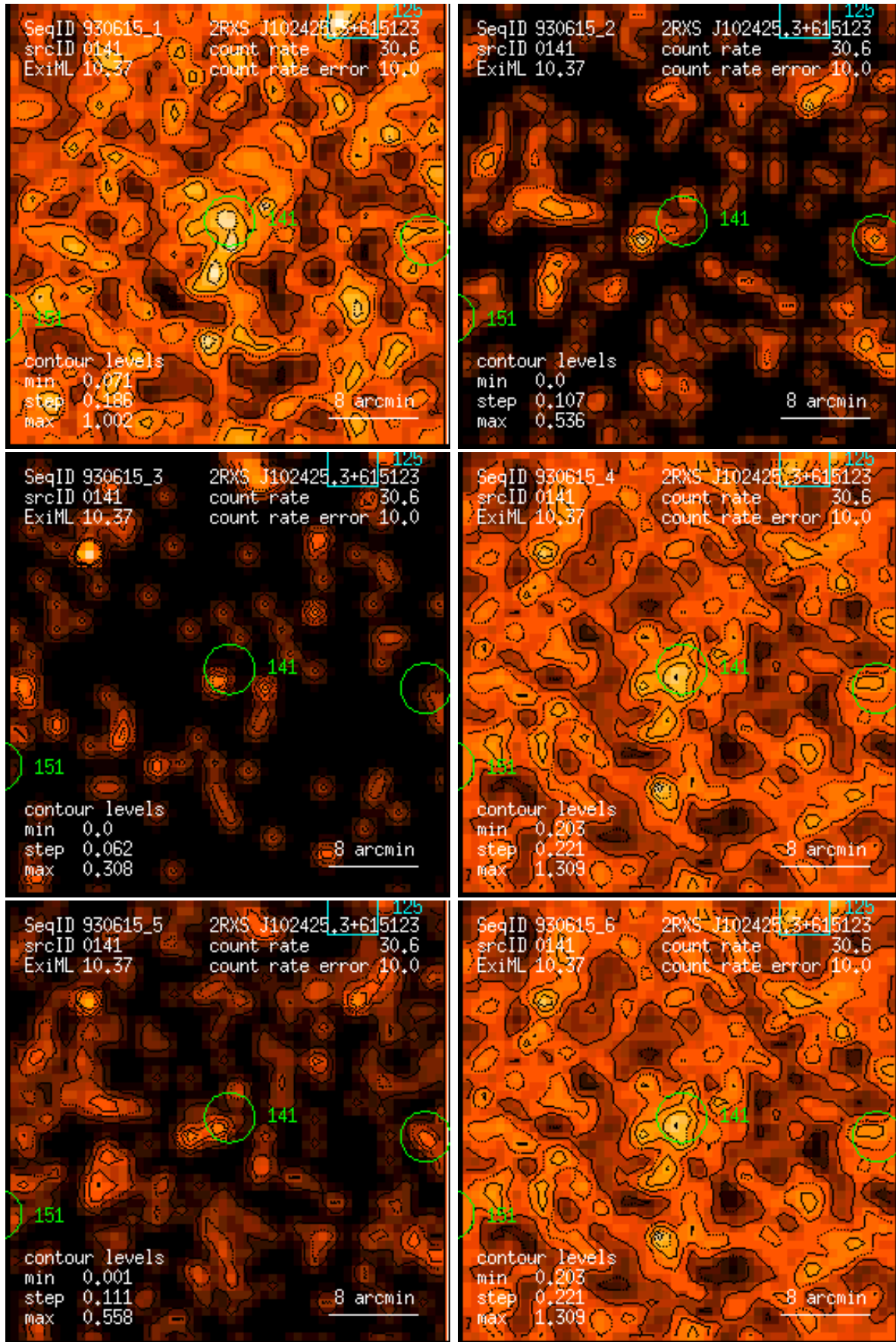
Figure 141: RASS 930615: detection 0141: band rate images, Gaussian filter: (1) PSPC channels 11 – 41, (2) 52 – 90, (3) 91 – 201, (4) 11 – 235, (5) 52 – 201, (6) 11 – 201. Broad band rates in counts/ks. Band rate contour levels in counts/ks/arcmin 2 .
