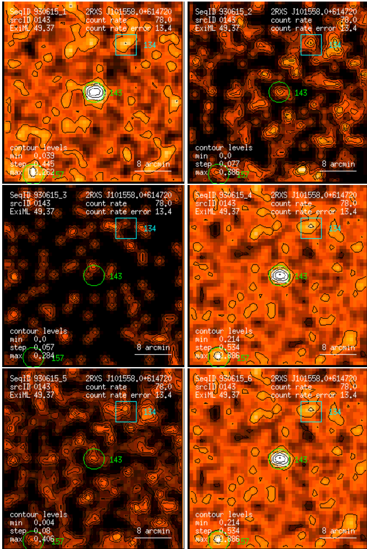
Figure 143: RASS 930615: detection 0143: band rate images, Gaussian filter: (1) PSPC channels 11 – 41, (2) 52 – 90, (3) 91 – 201, (4) 11 – 235, (5) 52 – 201, (6) 11 – 201. Broad band rates in counts/ks. Band rate contour levels in counts/ks/arcmin 2 .
