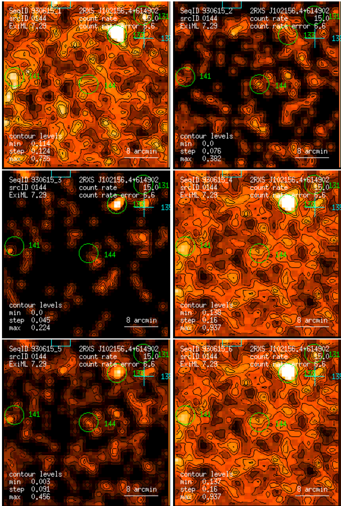
Figure 144: RASS 930615: detection 0144: band rate images, Gaussian filter: (1) PSPC channels 11 – 41, (2) 52 – 90, (3) 91 – 201, (4) 11 – 235, (5) 52 – 201, (6) 11 – 201. Broad band rates in counts/ks. Band rate contour levels in counts/ks/arcmin 2 .
