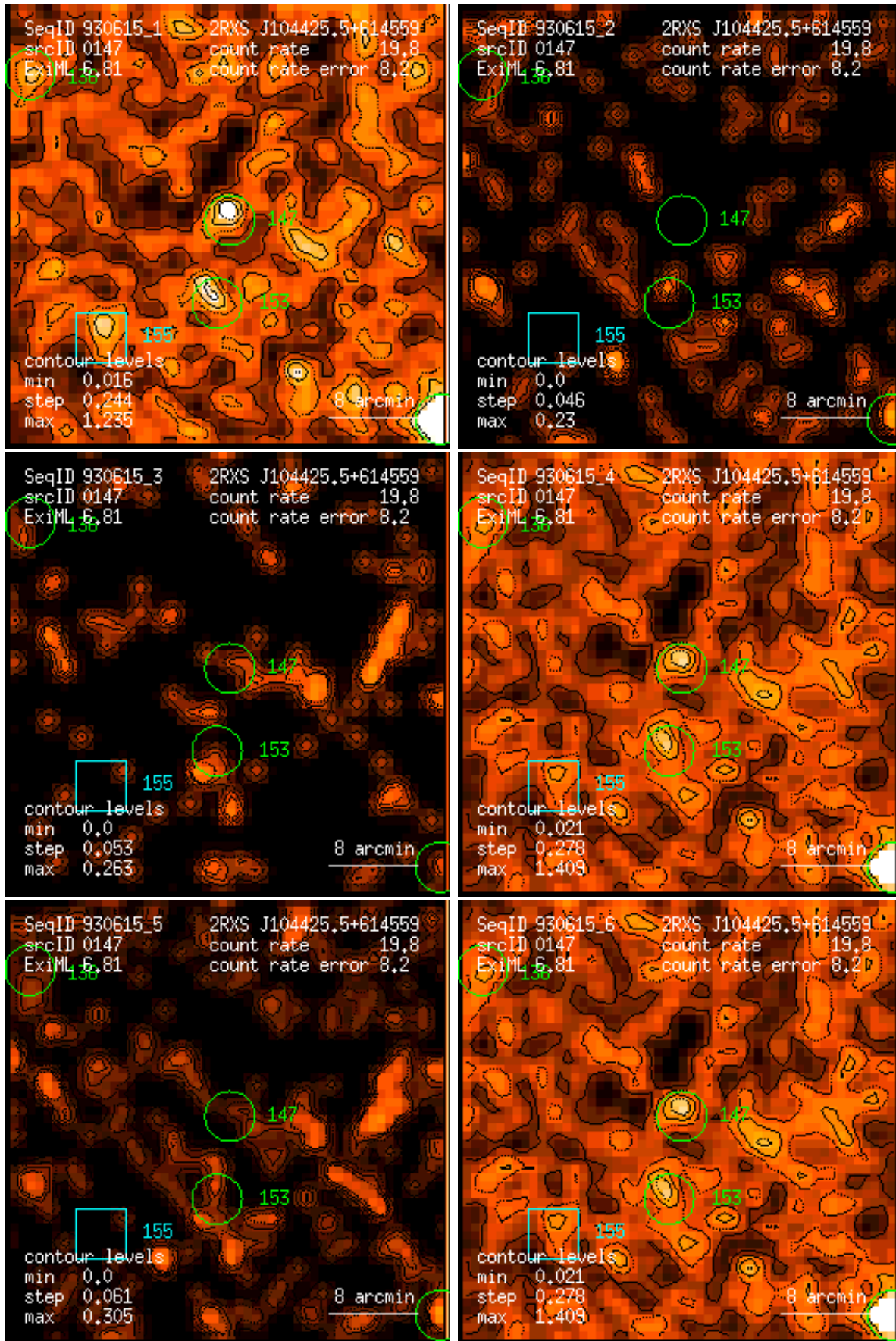
Figure 147: RASS 930615: detection 0147: band rate images, Gaussian filter: (1) PSPC channels 11 – 41, (2) 52 – 90, (3) 91 – 201, (4) 11 – 235, (5) 52 – 201, (6) 11 – 201. Broad band rates in counts/ks. Band rate contour levels in counts/ks/arcmin 2 .
