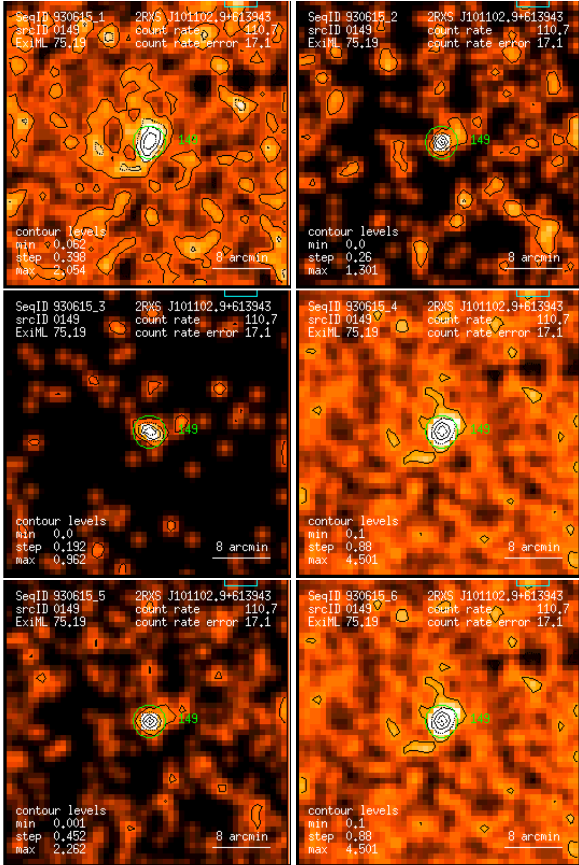
Figure 149: RASS 930615: detection 0149: band rate images, Gaussian filter: (1) PSPC channels 11 – 41, (2) 52 – 90, (3) 91 – 201, (4) 11 – 235, (5) 52 – 201, (6) 11 – 201. Broad band rates in counts/ks. Band rate contour levels in counts/ks/arcmin 2 .
