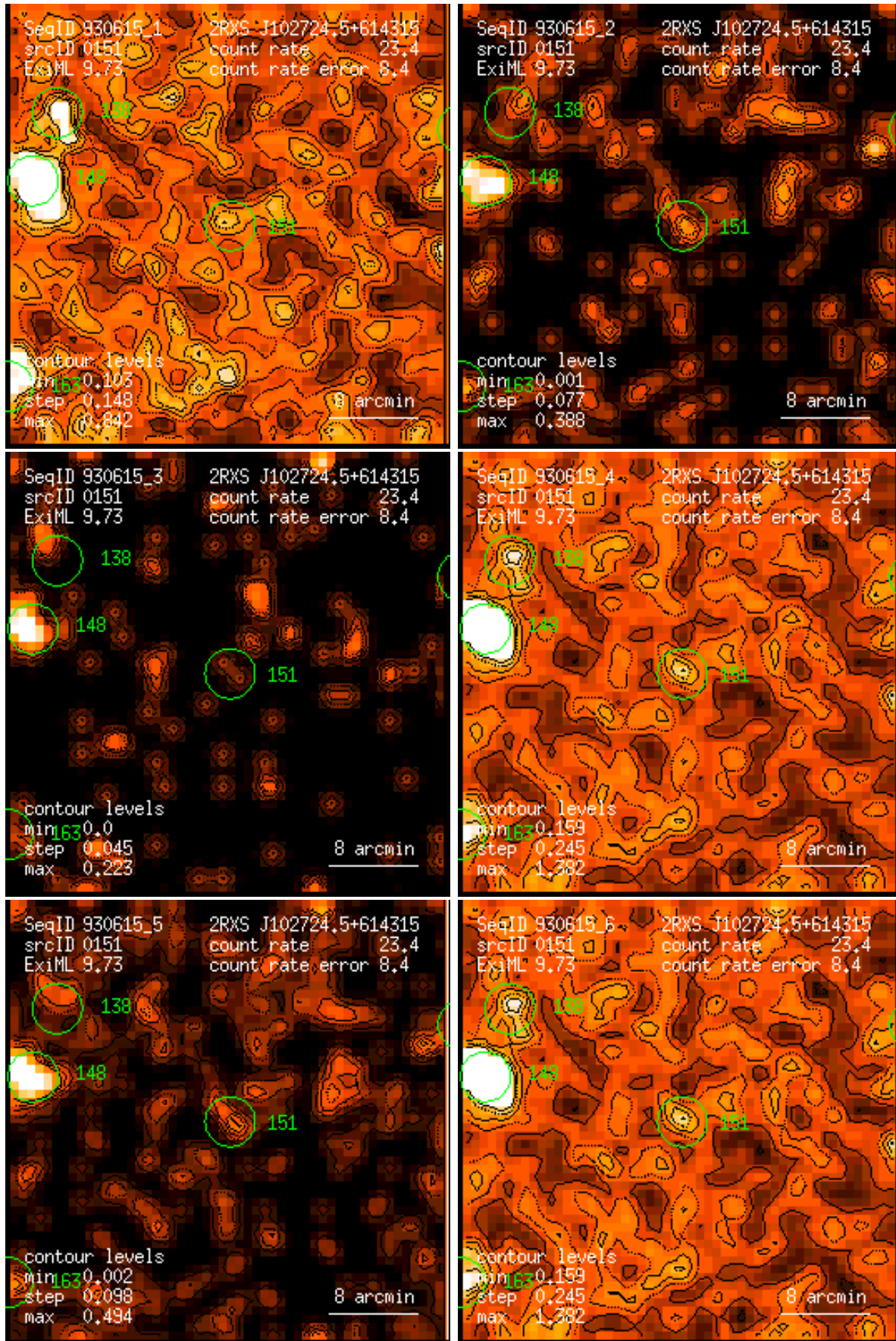
Figure 151: RASS 930615: detection 0151: band rate images, Gaussian filter: (1) PSPC channels 11 – 41, (2) 52 – 90, (3) 91 – 201, (4) 11 – 235, (5) 52 – 201, (6) 11 – 201. Broad band rates in counts/ks. Band rate contour levels in counts/ks/arcmin 2 .
