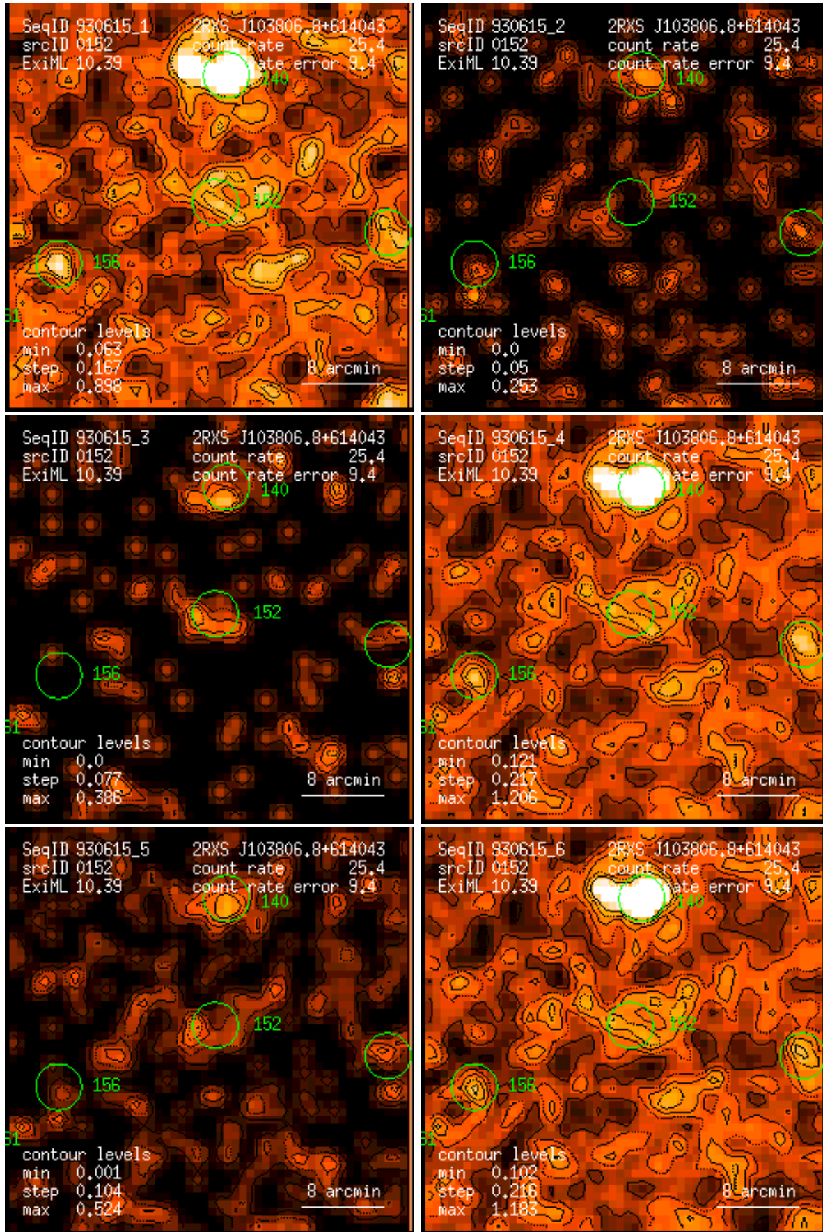
Figure 152: RASS 930615: detection 0152: band rate images, Gaussian filter: (1) PSPC channels 11 – 41, (2) 52 – 90, (3) 91 – 201, (4) 11 – 235, (5) 52 – 201, (6) 11 – 201. Broad band rates in counts/ks. Band rate contour levels in counts/ks/arcmin 2 .
