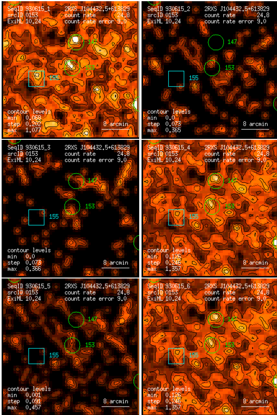
Figure 153: RASS 930615: detection 0153: band rate images, Gaussian filter: (1) PSPC channels 11 – 41, (2) 52 – 90, (3) 91 – 201, (4) 11 – 235, (5) 52 – 201, (6) 11 – 201. Broad band rates in counts/ks. Band rate contour levels in counts/ks/arcmin 2 .
