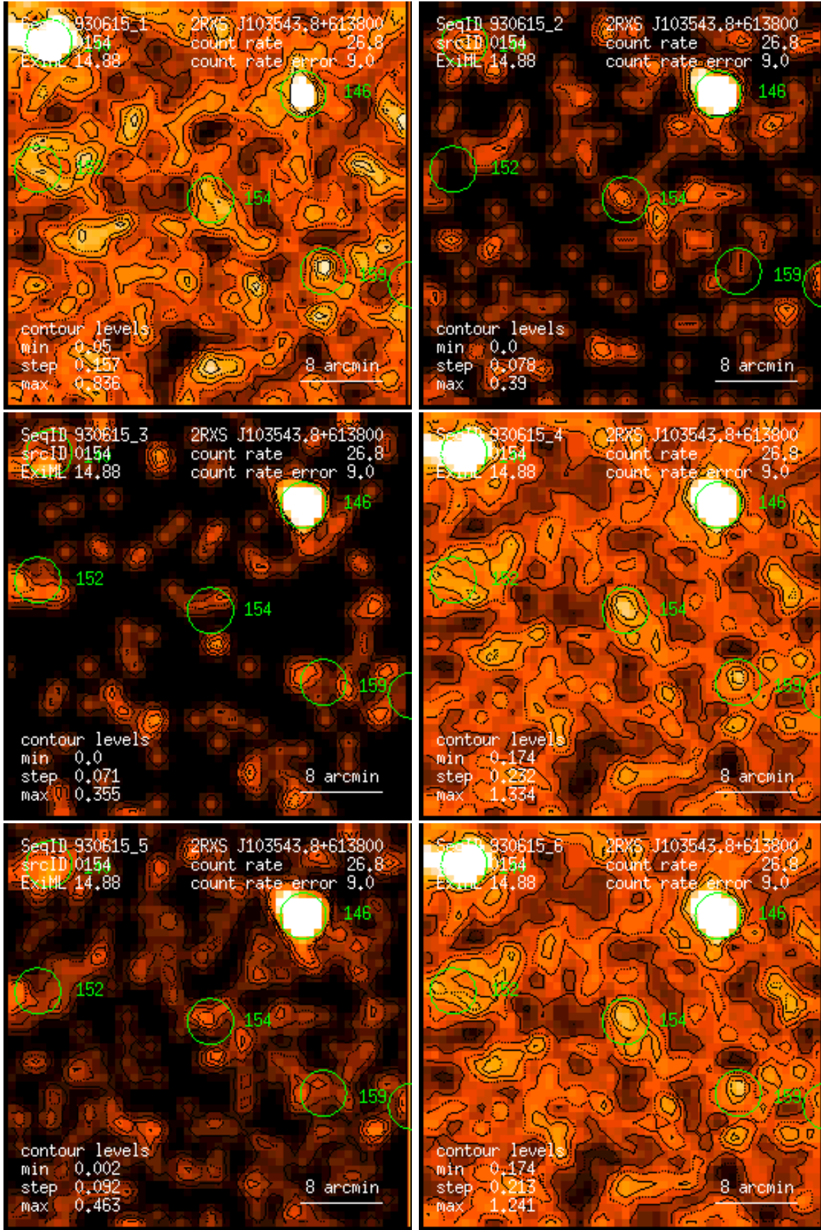
Figure 154: RASS 930615: detection 0154: band rate images, Gaussian filter: (1) PSPC channels 11 – 41, (2) 52 – 90, (3) 91 – 201, (4) 11 – 235, (5) 52 – 201, (6) 11 – 201. Broad band rates in counts/ks. Band rate contour levels in counts/ks/arcmin 2 .
