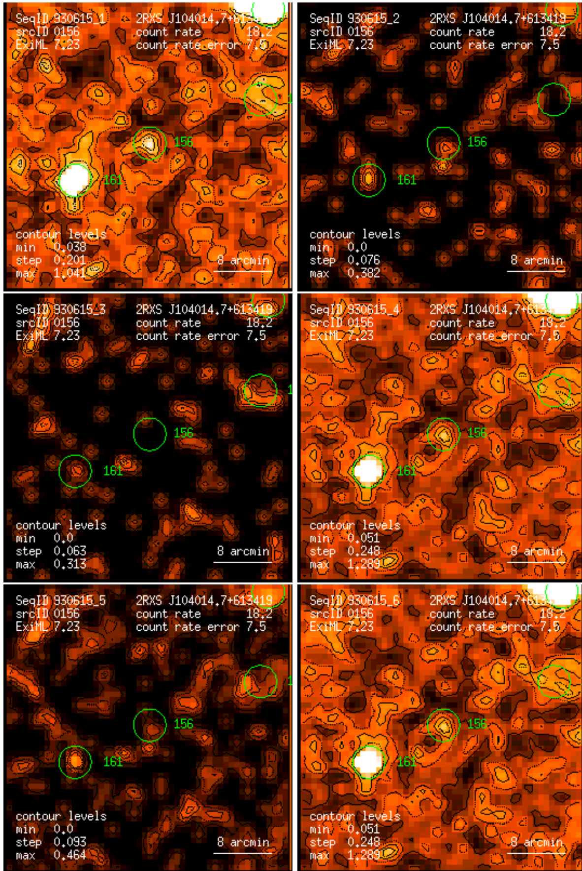
Figure 156: RASS 930615: detection 0156: band rate images, Gaussian filter: (1) PSPC channels 11 – 41, (2) 52 – 90, (3) 91 – 201, (4) 11 – 235, (5) 52 – 201, (6) 11 – 201. Broad band rates in counts/ks. Band rate contour levels in counts/ks/arcmin 2 .
