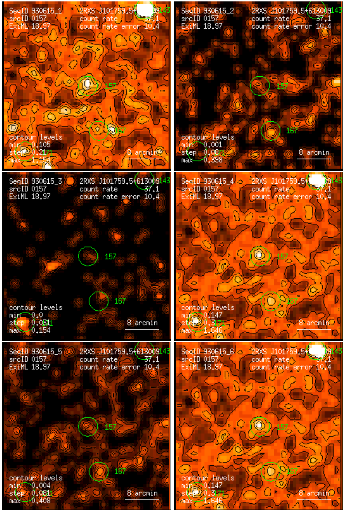
Figure 157: RASS 930615: detection 0157: band rate images, Gaussian filter: (1) PSPC channels 11 – 41, (2) 52 – 90, (3) 91 – 201, (4) 11 – 235, (5) 52 – 201, (6) 11 – 201. Broad band rates in counts/ks. Band rate contour levels in counts/ks/arcmin 2 .
