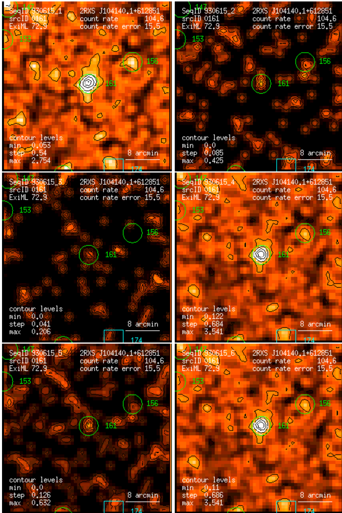
Figure 161: RASS 930615: detection 0161: band rate images, Gaussian filter: (1) PSPC channels 11 – 41, (2) 52 – 90, (3) 91 – 201, (4) 11 – 235, (5) 52 – 201, (6) 11 – 201. Broad band rates in counts/ks. Band rate contour levels in counts/ks/arcmin 2 .
