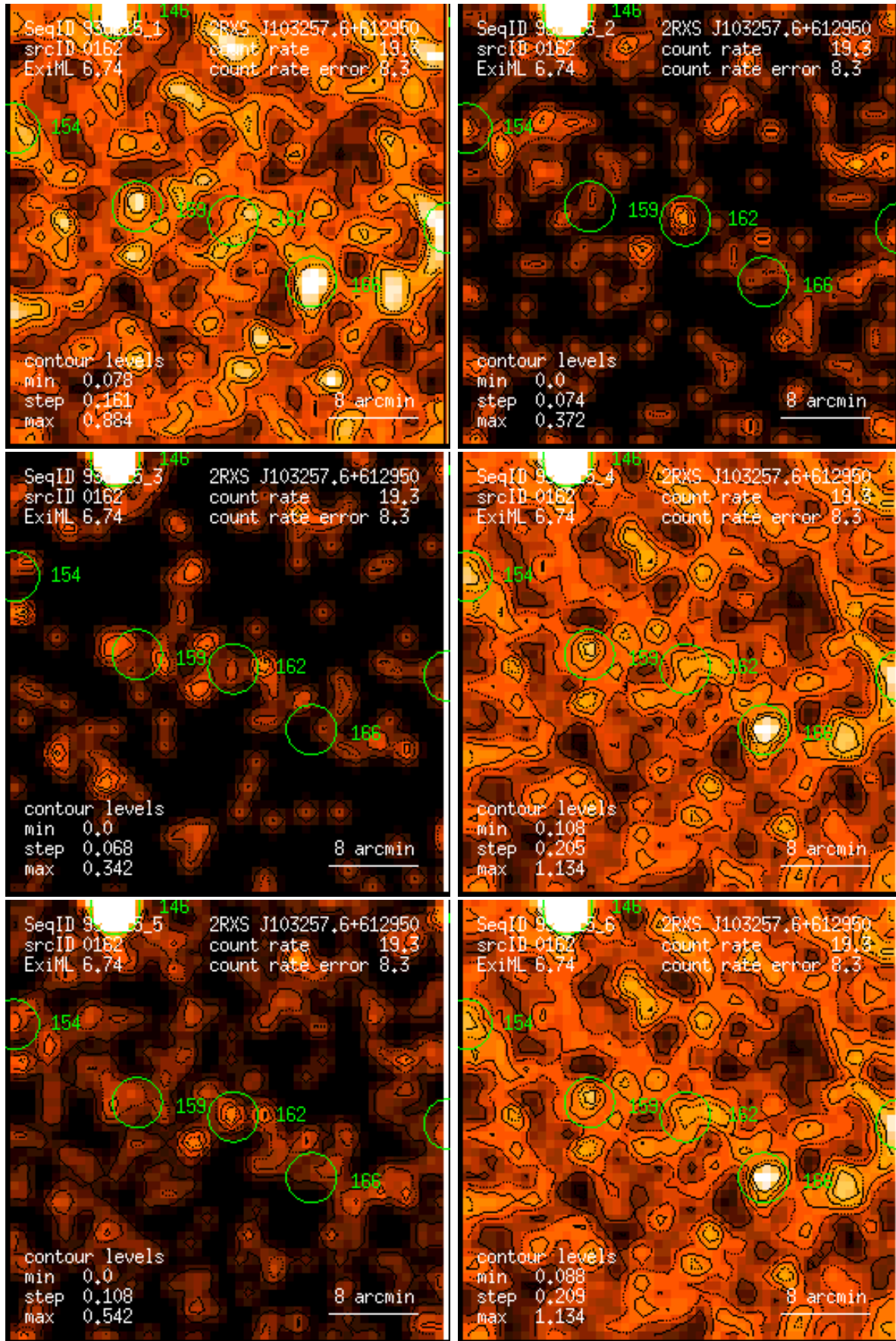
Figure 162: RASS 930615: detection 0162: band rate images, Gaussian filter: (1) PSPC channels 11 – 41, (2) 52 – 90, (3) 91 – 201, (4) 11 – 235, (5) 52 – 201, (6) 11 – 201. Broad band rates in counts/ks. Band rate contour levels in counts/ks/arcmin 2 .
