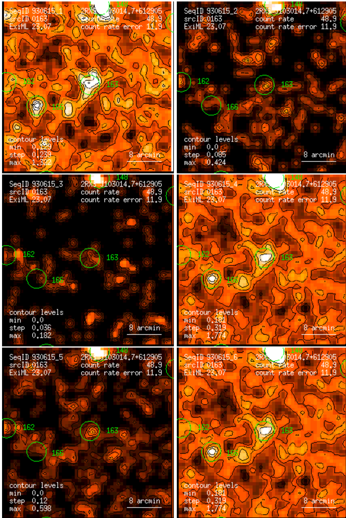
Figure 163: RASS 930615: detection 0163: band rate images, Gaussian filter: (1) PSPC channels 11 – 41, (2) 52 – 90, (3) 91 – 201, (4) 11 – 235, (5) 52 – 201, (6) 11 – 201. Broad band rates in counts/ks. Band rate contour levels in counts/ks/arcmin 2 .
