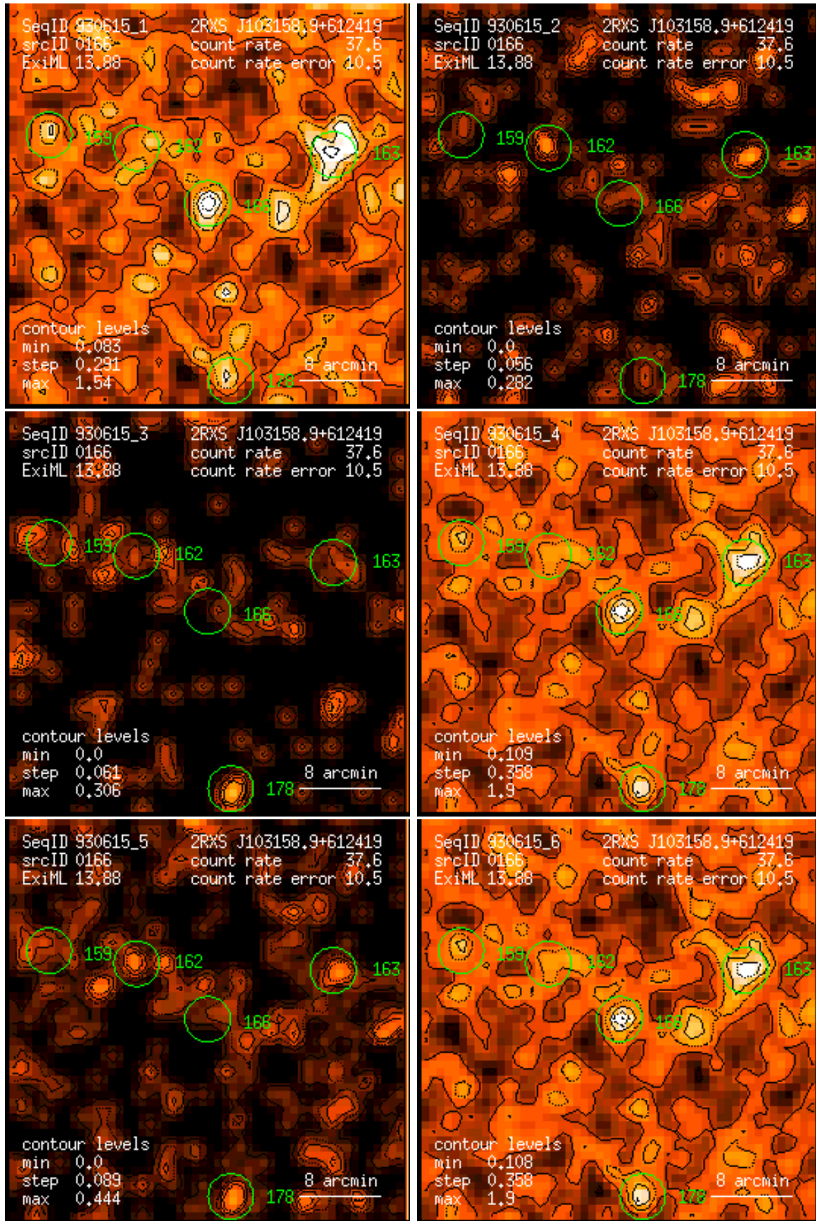
Figure 166: RASS 930615: detection 0166: band rate images, Gaussian filter: (1) PSPC channels 11 – 41, (2) 52 – 90, (3) 91 – 201, (4) 11 – 235, (5) 52 – 201, (6) 11 – 201. Broad band rates in counts/ks. Band rate contour levels in counts/ks/arcmin 2 .
