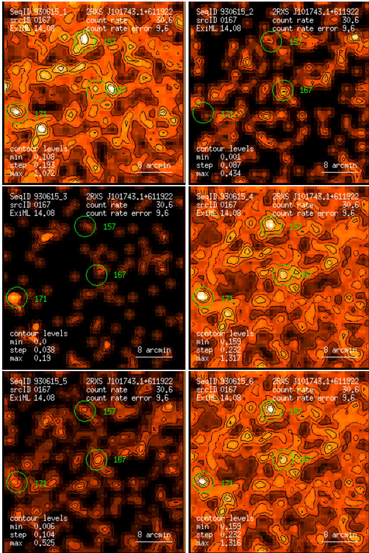
Figure 167: RASS 930615: detection 0167: band rate images, Gaussian filter: (1) PSPC channels 11 – 41, (2) 52 – 90, (3) 91 – 201, (4) 11 – 235, (5) 52 – 201, (6) 11 – 201. Broad band rates in counts/ks. Band rate contour levels in counts/ks/arcmin 2 .
