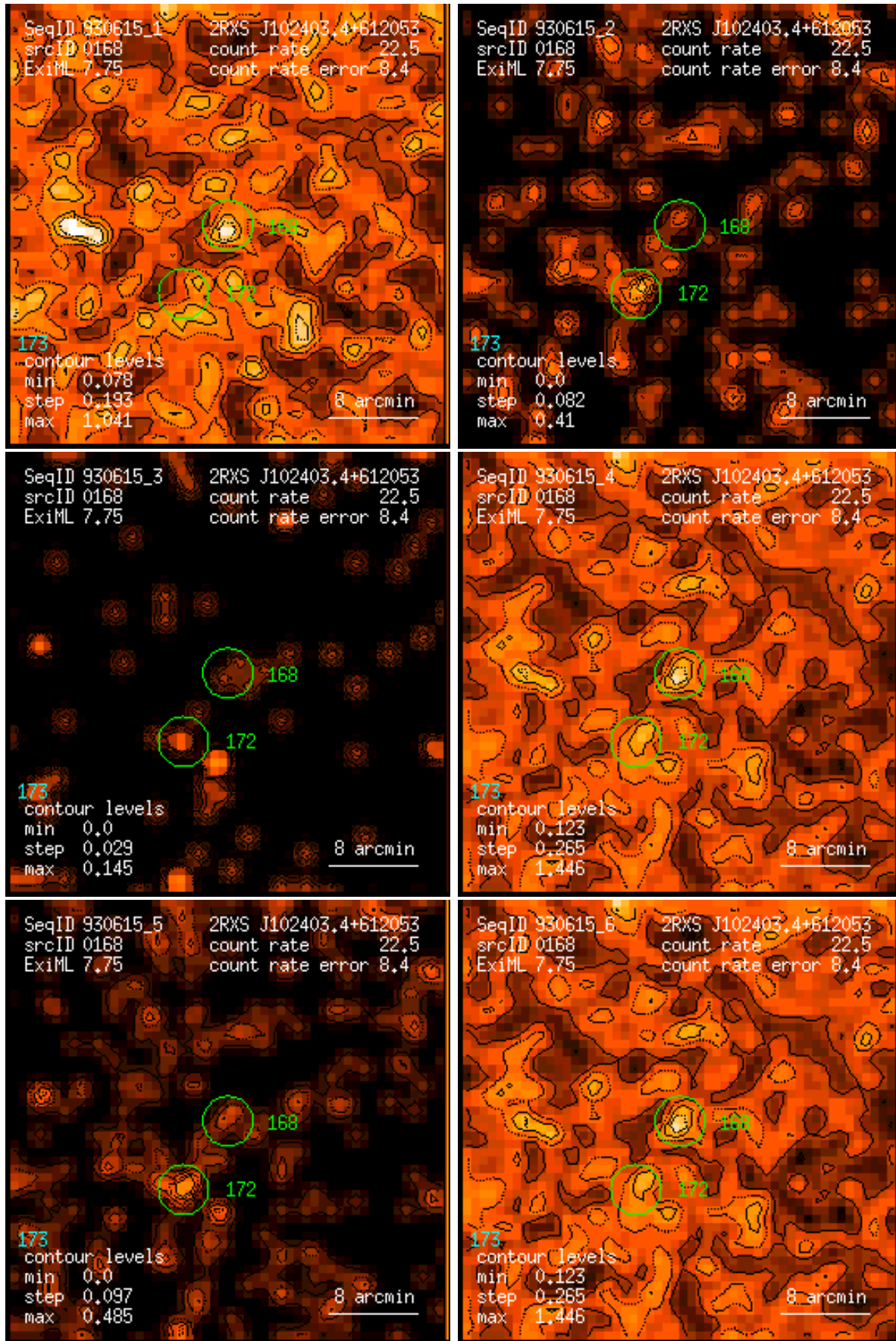
Figure 168: RASS 930615: detection 0168: band rate images, Gaussian filter: (1) PSPC channels 11 – 41, (2) 52 – 90, (3) 91 – 201, (4) 11 – 235, (5) 52 – 201, (6) 11 – 201. Broad band rates in counts/ks. Band rate contour levels in counts/ks/arcmin 2 .
