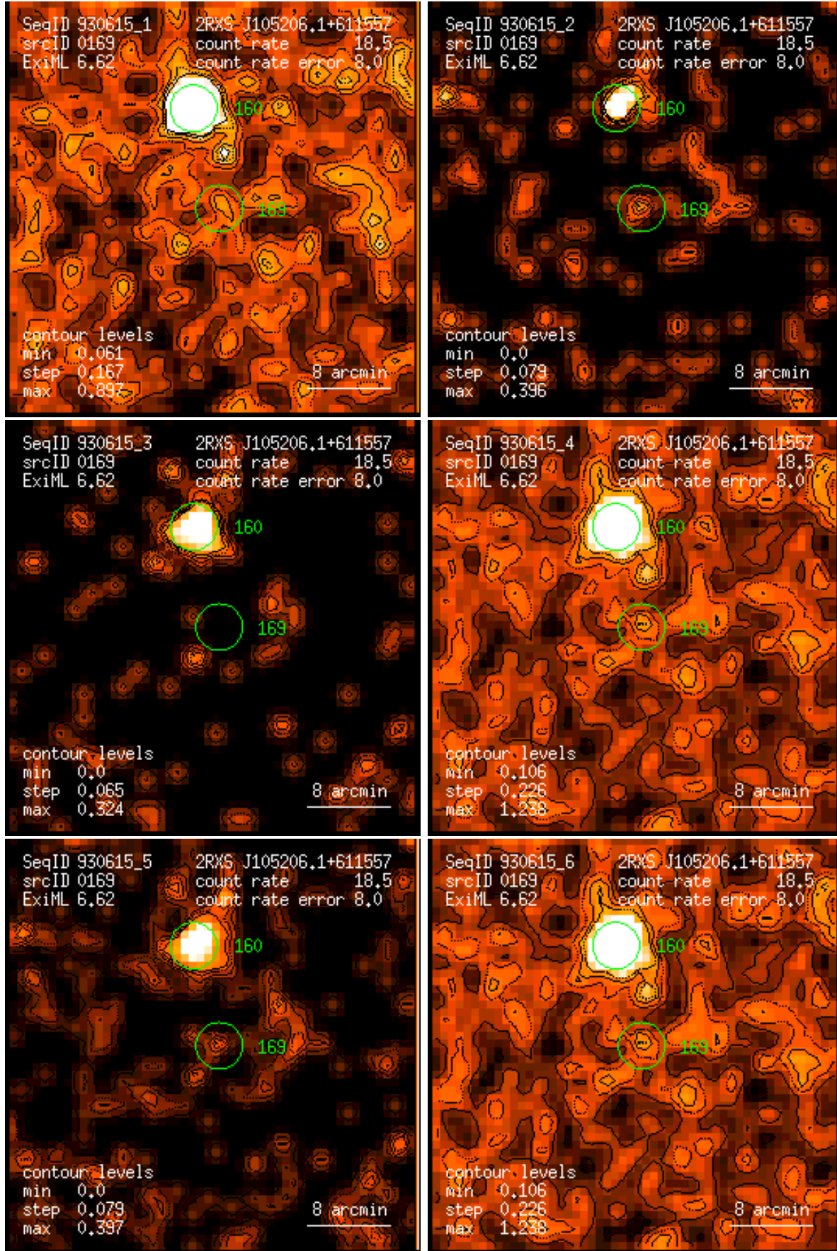
Figure 169: RASS 930615: detection 0169: band rate images, Gaussian filter: (1) PSPC channels 11 – 41, (2) 52 – 90, (3) 91 – 201, (4) 11 – 235, (5) 52 – 201, (6) 11 – 201. Broad band rates in counts/ks. Band rate contour levels in counts/ks/arcmin 2 .
