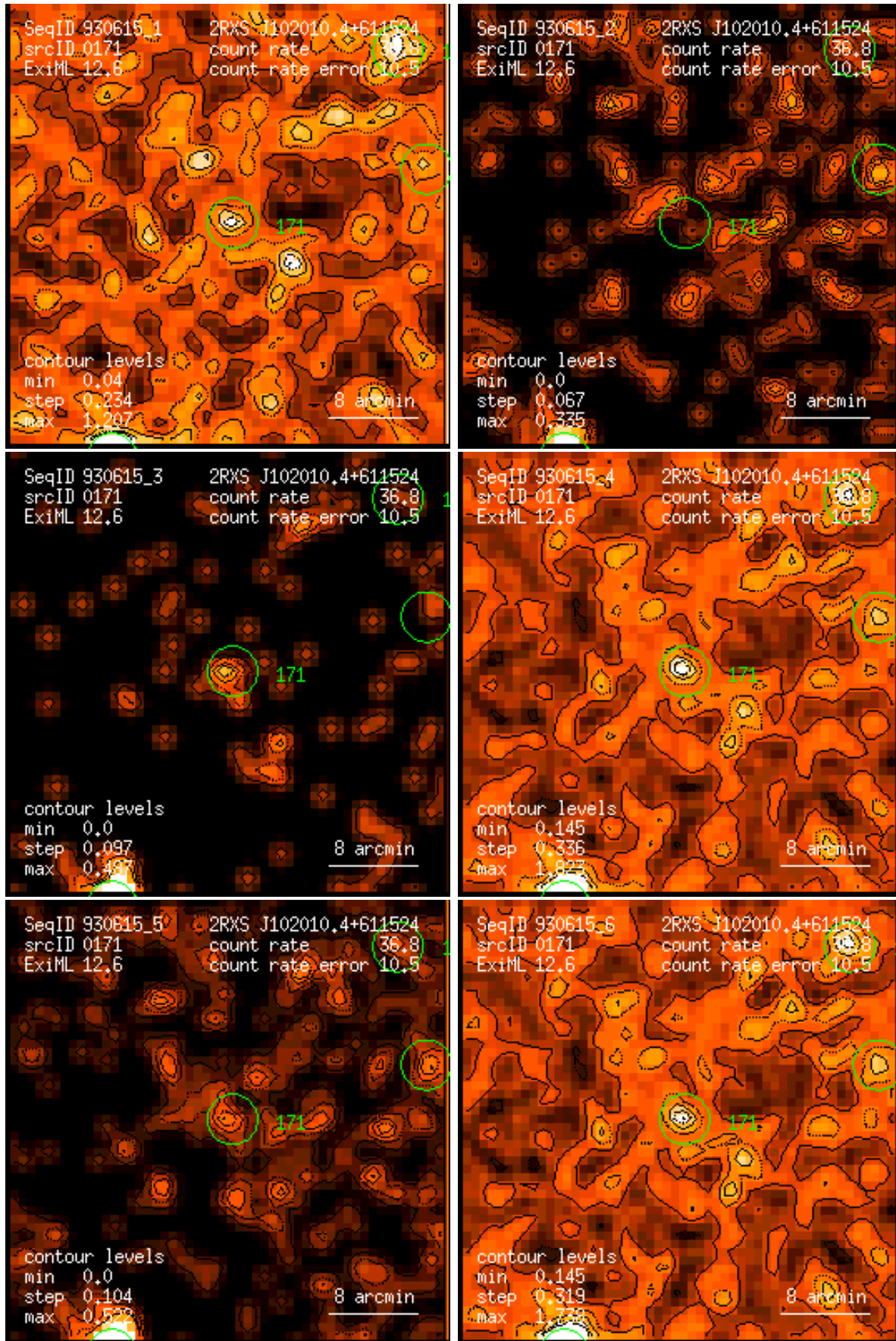
Figure 171: RASS 930615: detection 0171: band rate images, Gaussian filter: (1) PSPC channels 11 – 41, (2) 52 – 90, (3) 91 – 201, (4) 11 – 235, (5) 52 – 201, (6) 11 – 201. Broad band rates in counts/ks. Band rate contour levels in counts/ks/arcmin 2 .
