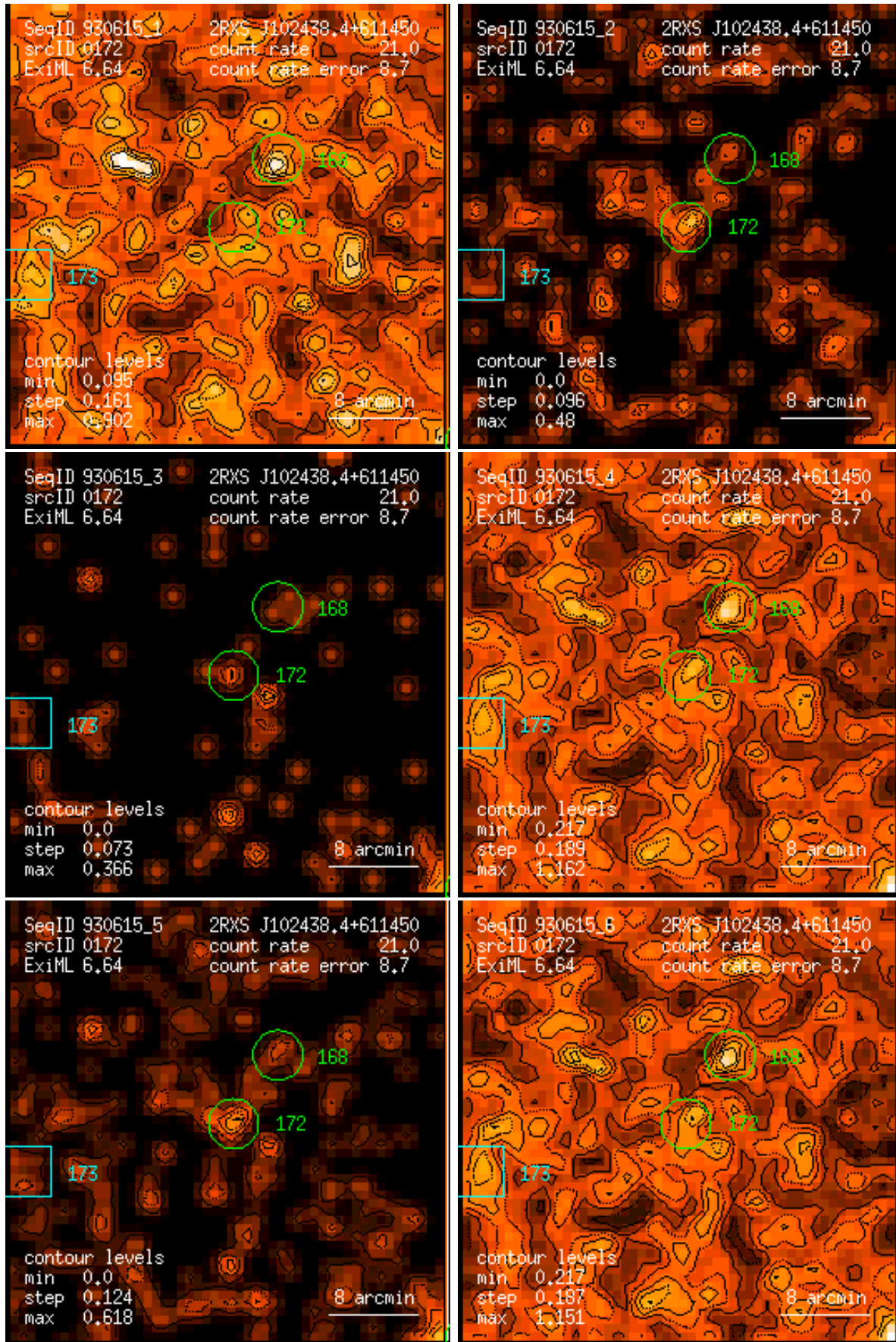
Figure 172: RASS 930615: detection 0172: band rate images, Gaussian filter: (1) PSPC channels 11 – 41, (2) 52 – 90, (3) 91 – 201, (4) 11 – 235, (5) 52 – 201, (6) 11 – 201. Broad band rates in counts/ks. Band rate contour levels in counts/ks/arcmin 2 .
