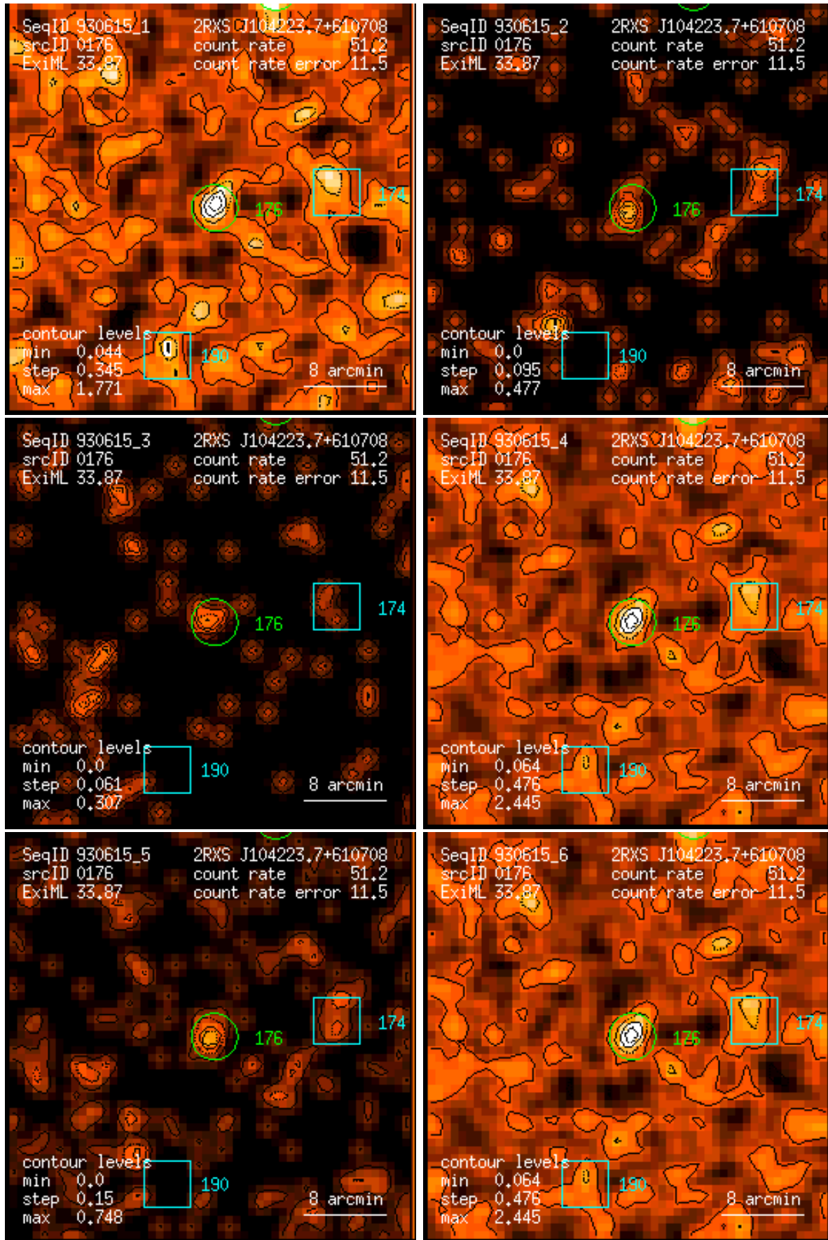
Figure 176: RASS 930615: detection 0176: band rate images, Gaussian filter: (1) PSPC channels 11 – 41, (2) 52 – 90, (3) 91 – 201, (4) 11 – 235, (5) 52 – 201, (6) 11 – 201. Broad band rates in counts/ks. Band rate contour levels in counts/ks/arcmin 2 .
