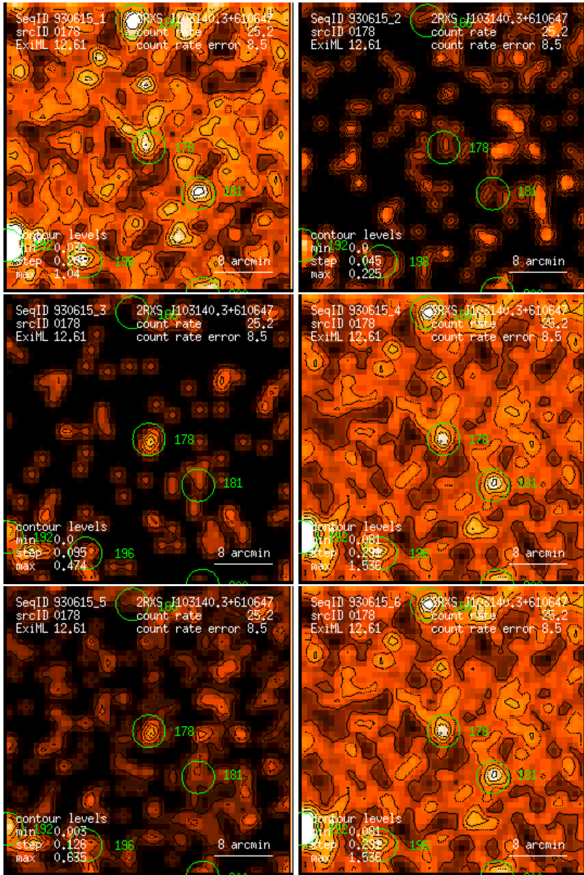
Figure 178: RASS 930615: detection 0178: band rate images, Gaussian filter: (1) PSPC channels 11 – 41, (2) 52 – 90, (3) 91 – 201, (4) 11 – 235, (5) 52 – 201, (6) 11 – 201. Broad band rates in counts/ks. Band rate contour levels in counts/ks/arcmin 2 .
