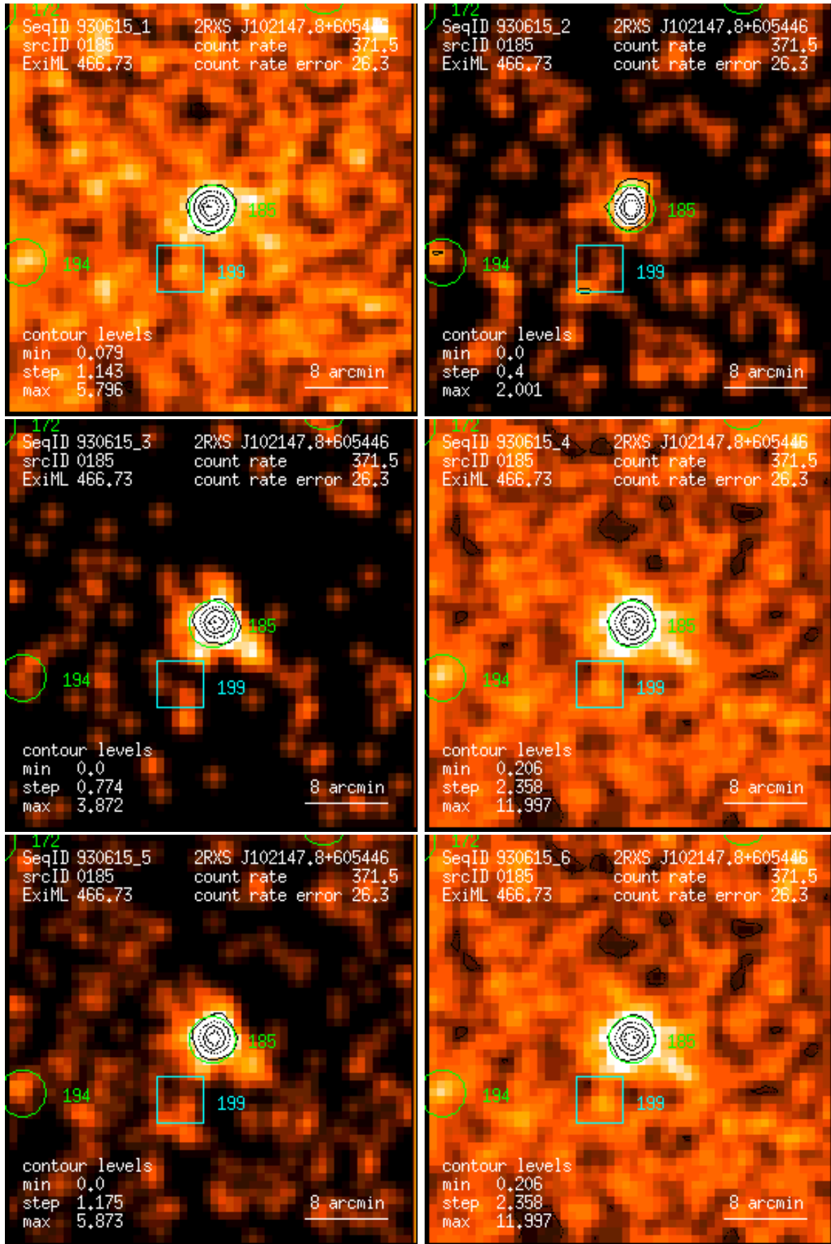
Figure 185: RASS 930615: detection 0185: band rate images, Gaussian filter: (1) PSPC channels 11 – 41, (2) 52 – 90, (3) 91 – 201, (4) 11 – 235, (5) 52 – 201, (6) 11 – 201. Broad band rates in counts/ks. Band rate contour levels in counts/ks/arcmin 2 .
