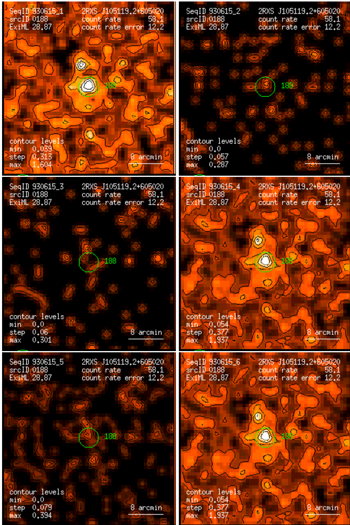
Figure 188: RASS 930615: detection 0188: band rate images, Gaussian filter: (1) PSPC channels 11 – 41, (2) 52 – 90, (3) 91 – 201, (4) 11 – 235, (5) 52 – 201, (6) 11 – 201. Broad band rates in counts/ks. Band rate contour levels in counts/ks/arcmin 2 .
